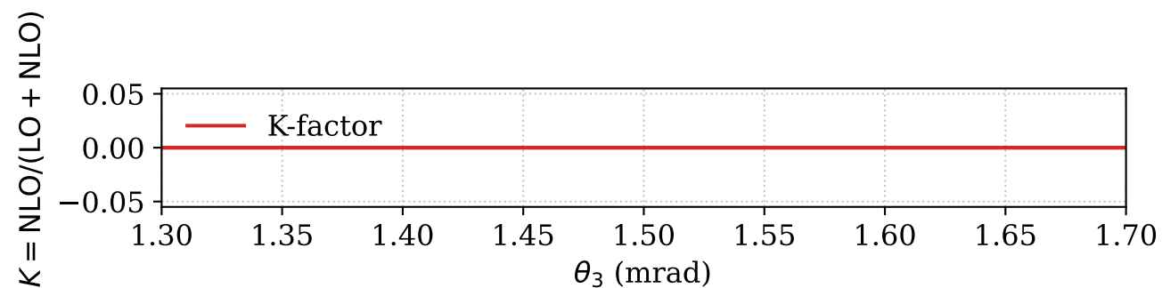
Photon Scattering Angle (cms)
