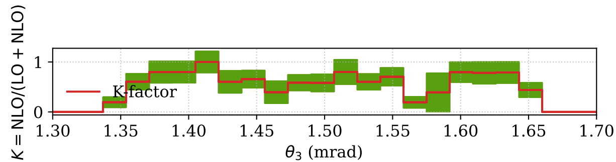
Photon Scattering Angle (lab)
