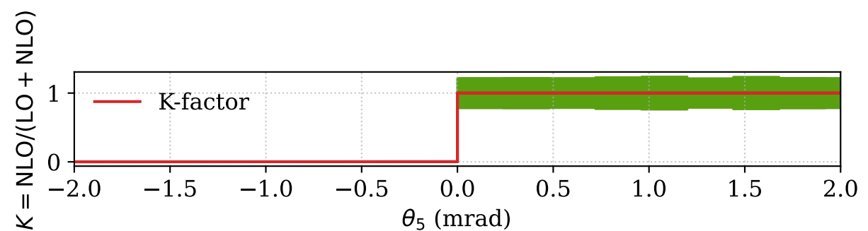
Photon Deflection Angle (lab)
