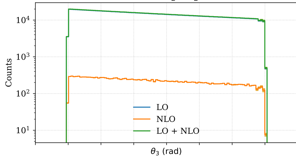
Scattering Angle
