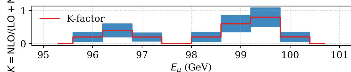
Photon Energy (lab)
