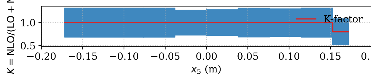
K = \text{NLO}/(\text{LO} + \text{NLO})
