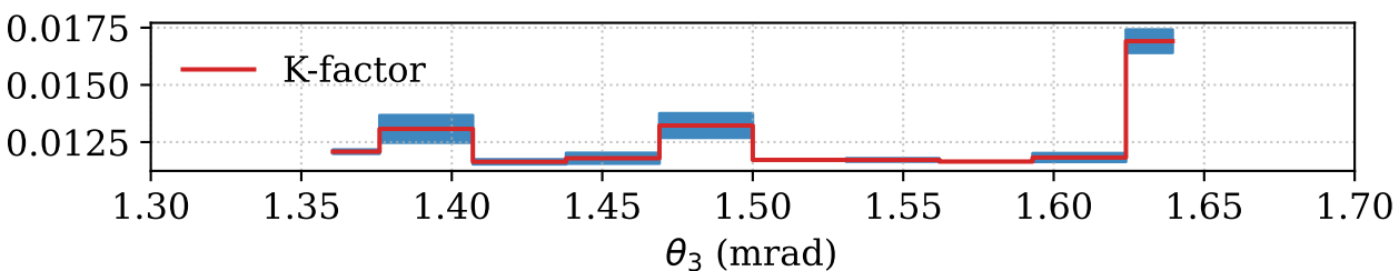
Photon Scattering Angle (lab)
