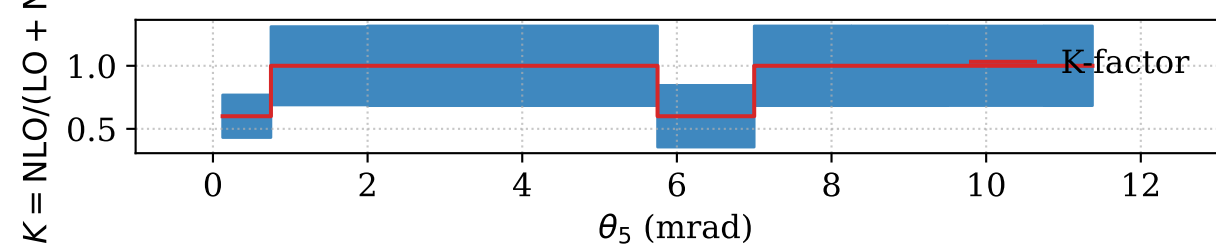
Photon Deflection Angle (lab)
