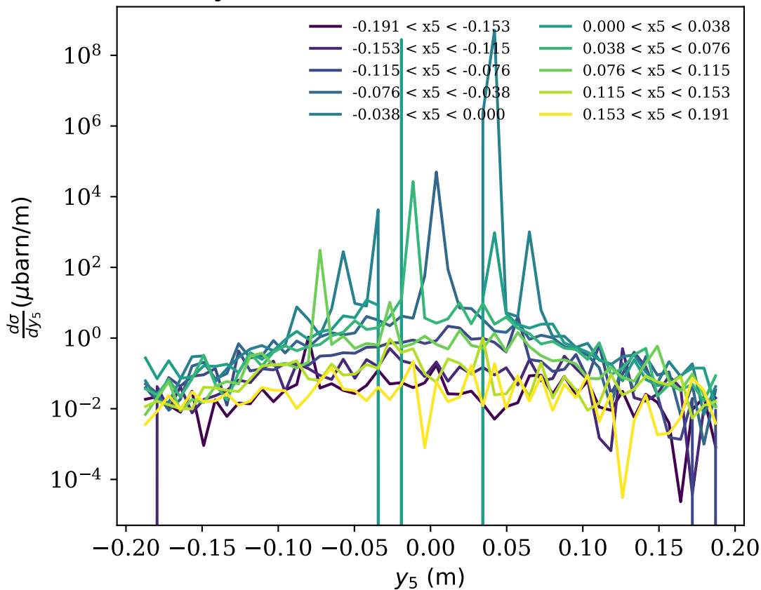
y5 distribution in x5-slices (lab)
