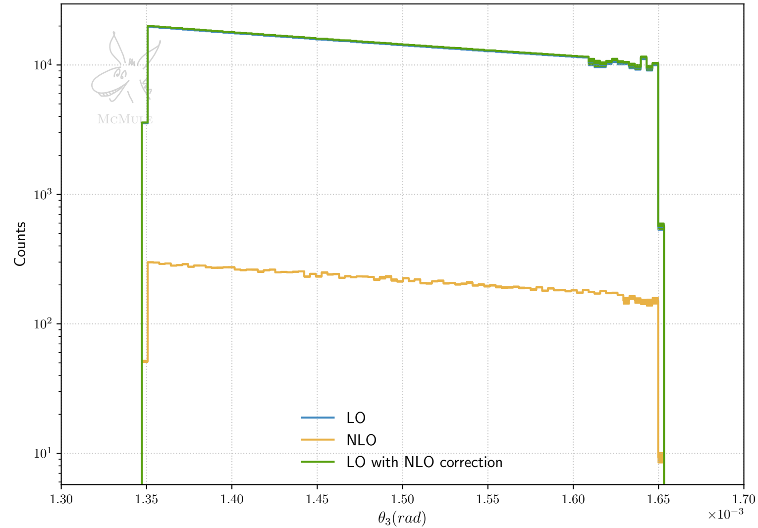
Scattering Angle
