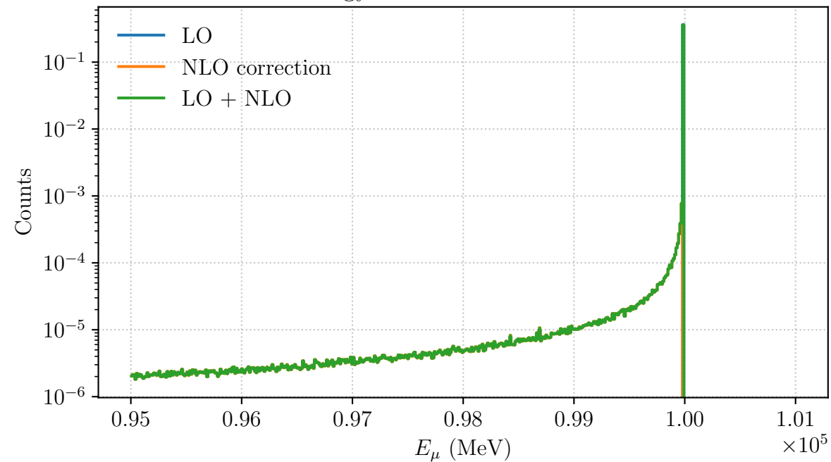
Energy of the Scattered Muon
