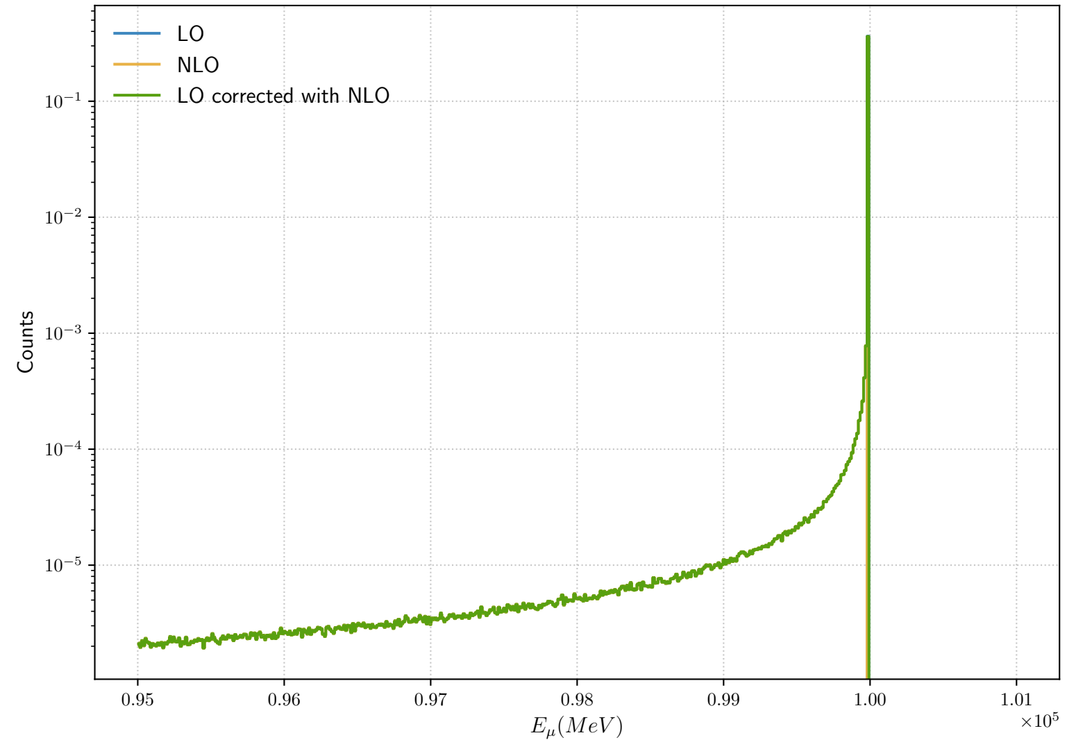
Energy of the Scattered Muon
