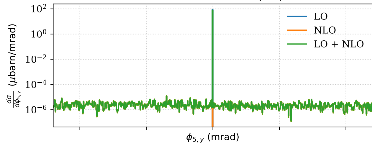
Photon Y-deflection (lab)
