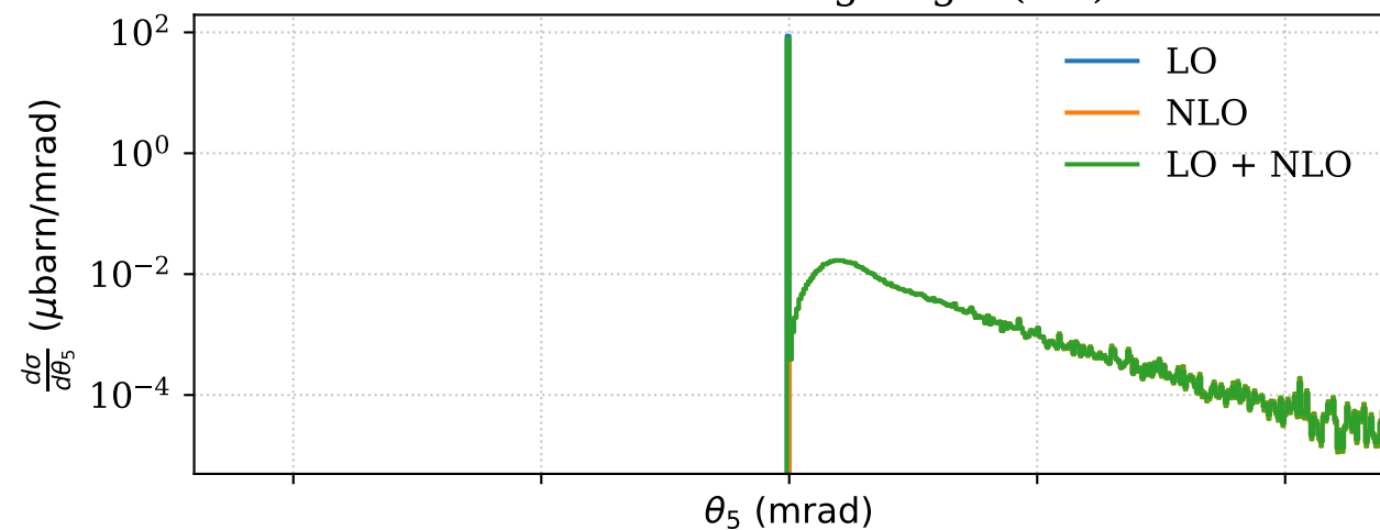
Photon Scattering Angle (lab)
