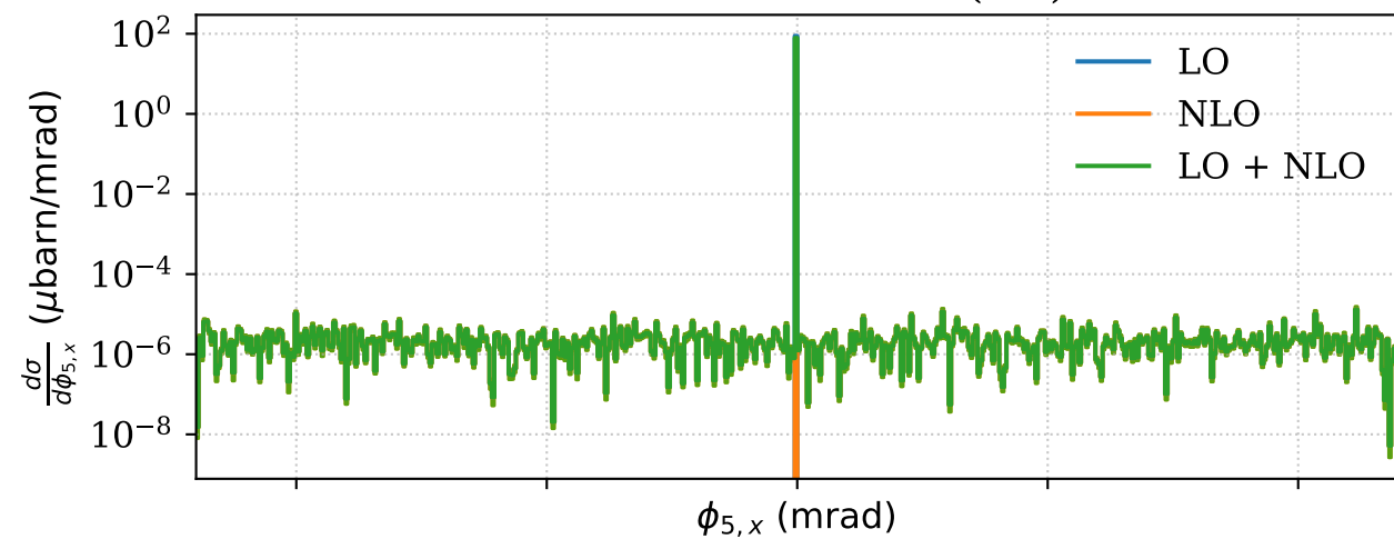
Photon X-deflection (lab)
