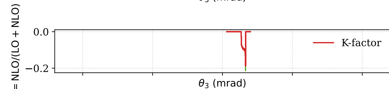
Photon Scattering Angle (lab)
