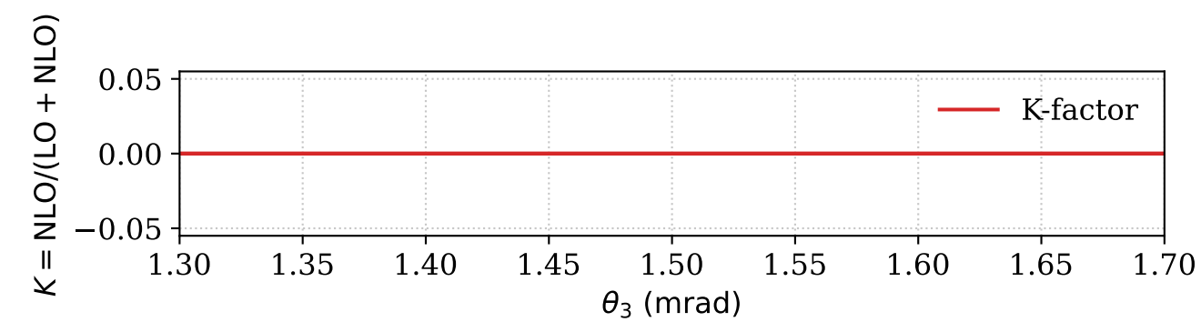
Photon Scattering Angle (cms)
