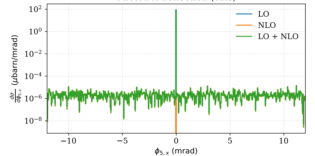
Photon X-deflection (cms)
