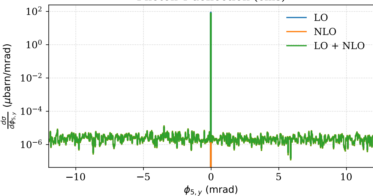
Photon Y-deflection (cms)
