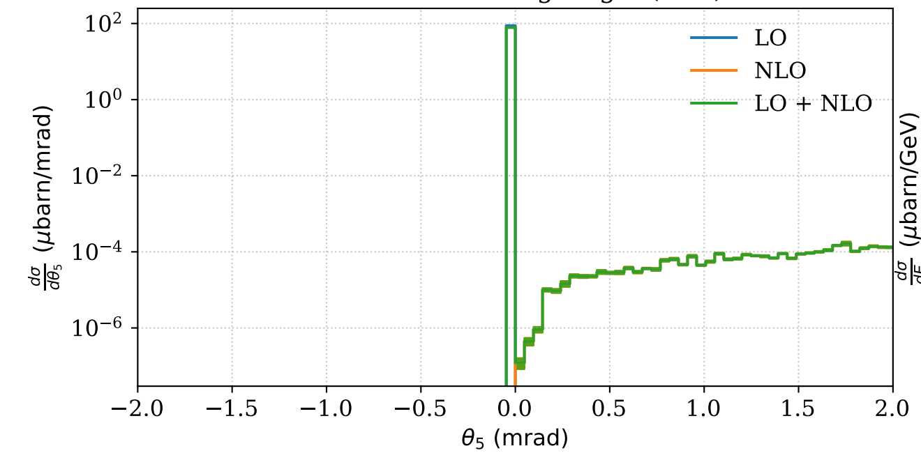
Photon Scattering Angle (cms)
