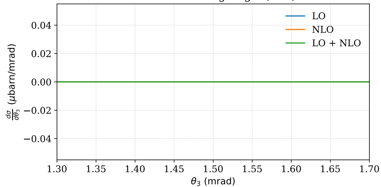
Muon Scattering Angle (cms)
