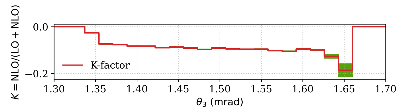
Photon Scattering Angle (lab)
