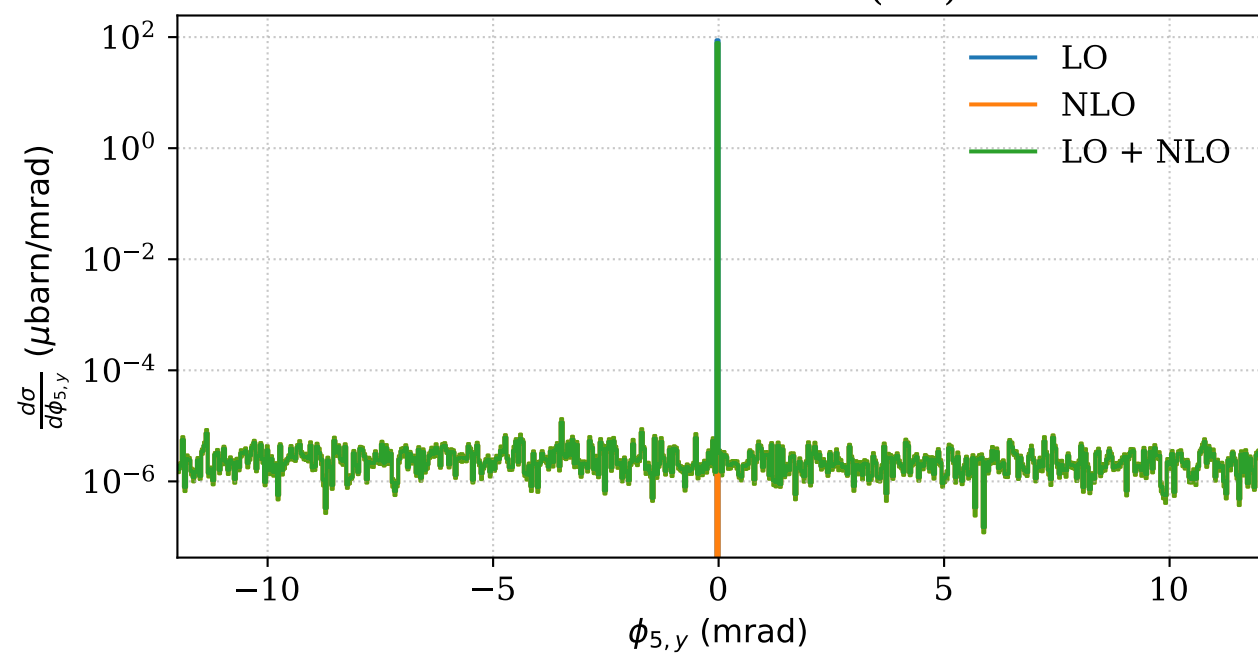
Photon Y-deflection (lab)
