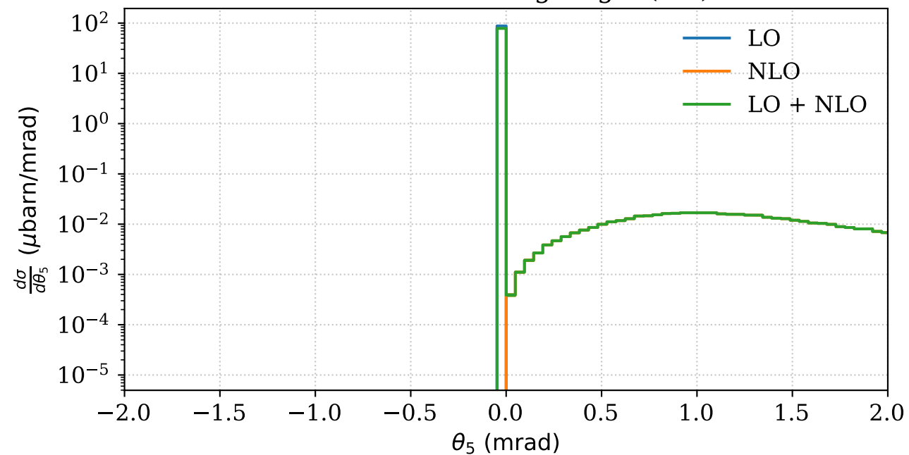
Photon Scattering Angle (lab)
