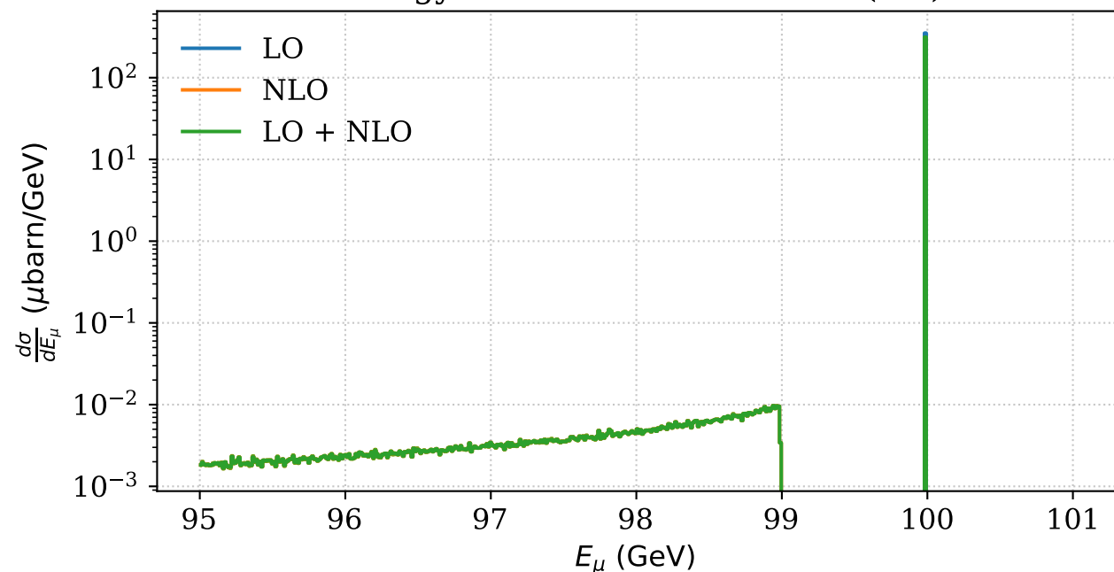
Energy of the Scattered Muon (lab)
