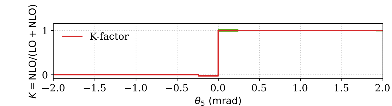
Photon X-deflection (lab)
