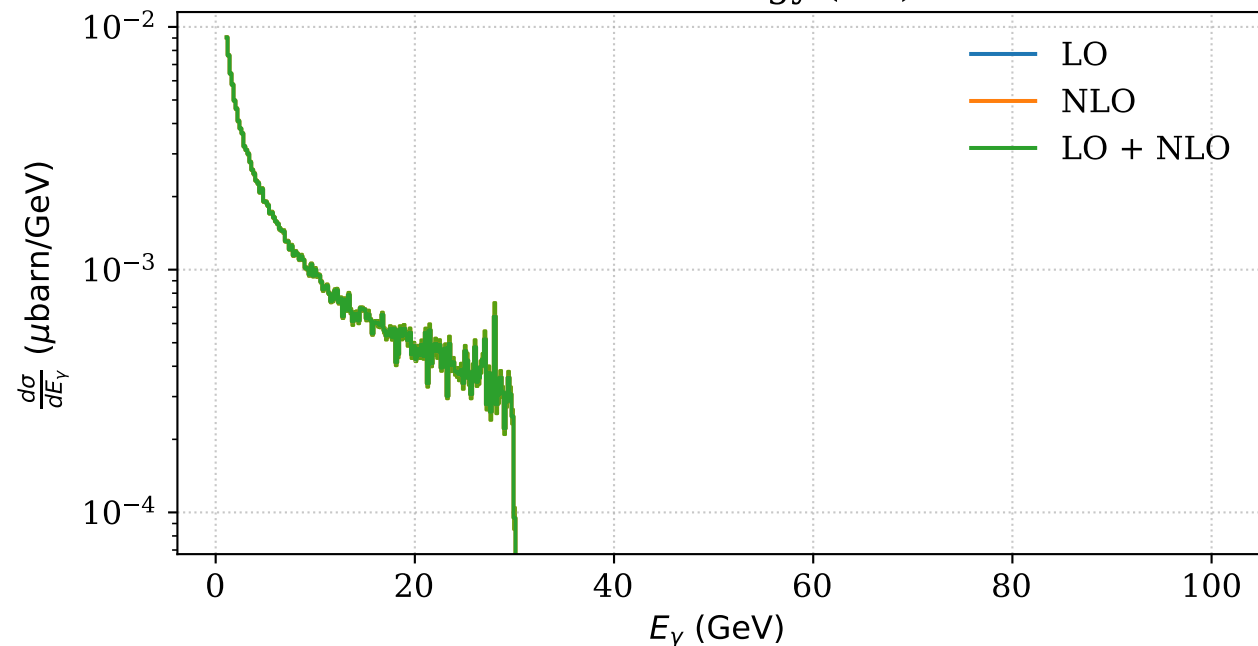
Photon Energy (lab)
