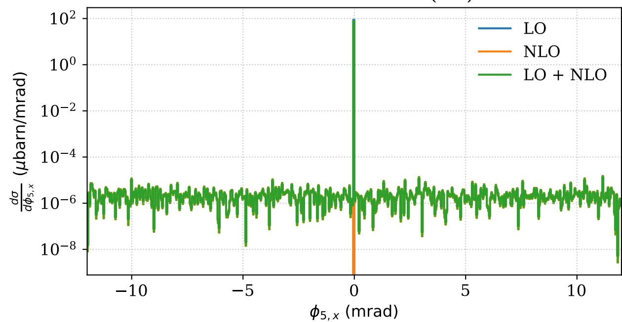
Photon X-deflection (lab)
