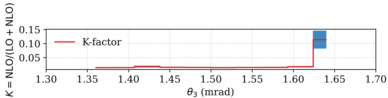
Photon Scattering Angle (lab)
