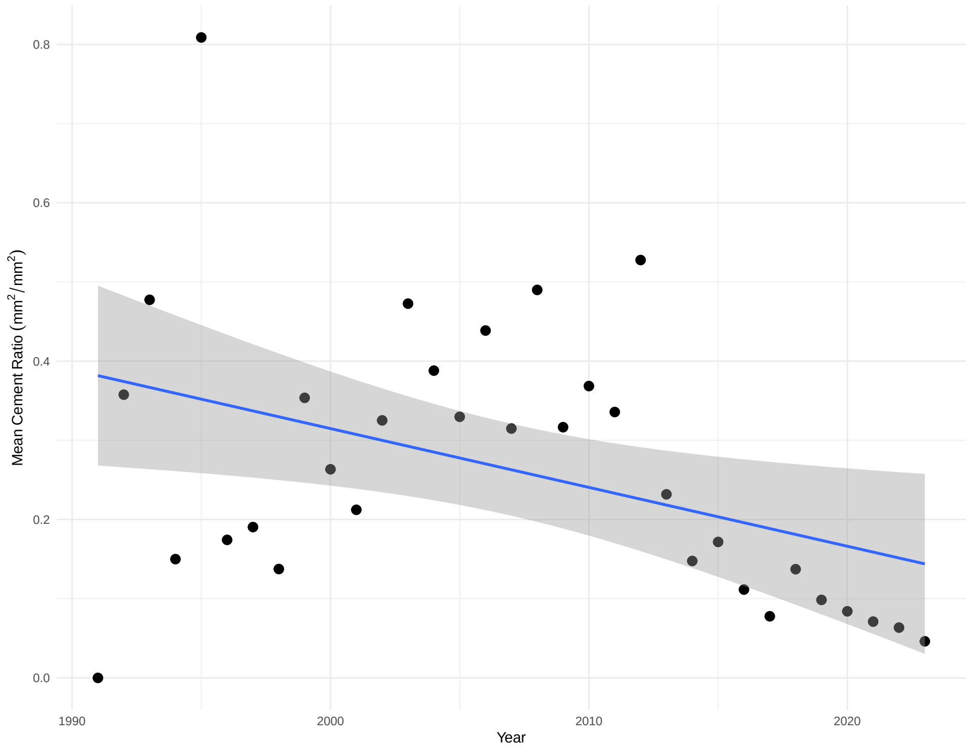
Mean Cement Ratio (without Sample 145)
