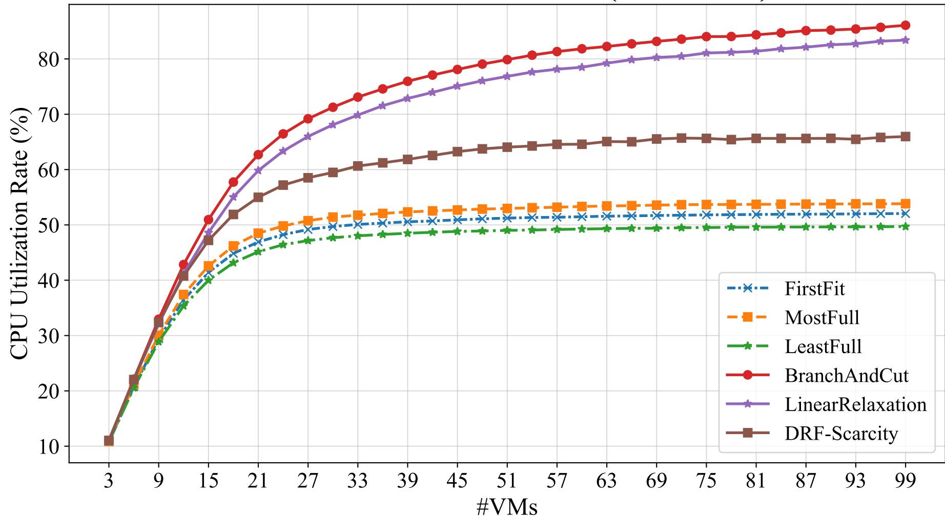
CPU Utilization Rate vs #VMs (over 3 Hosts)
