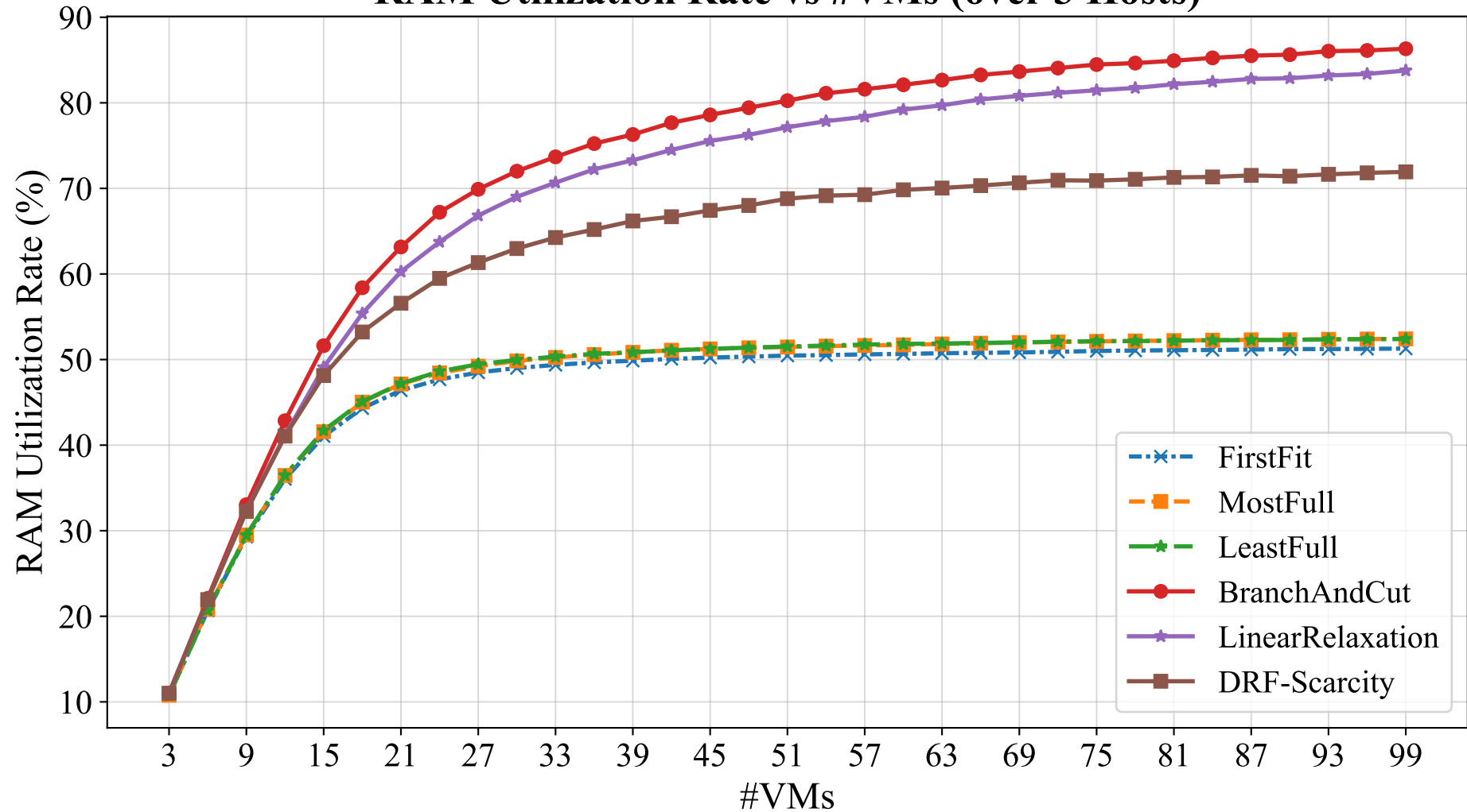
RAM Utilization Rate vs #VMs (over 3 Hosts)
