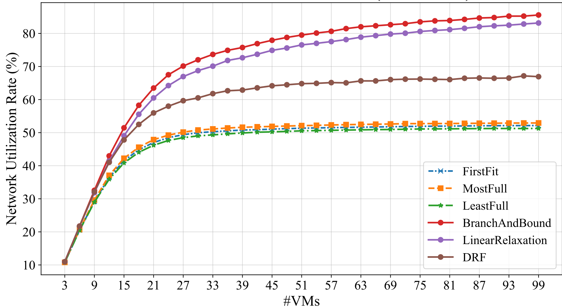
Network Utilization Rate vs #VMs (over 4 Hosts)
