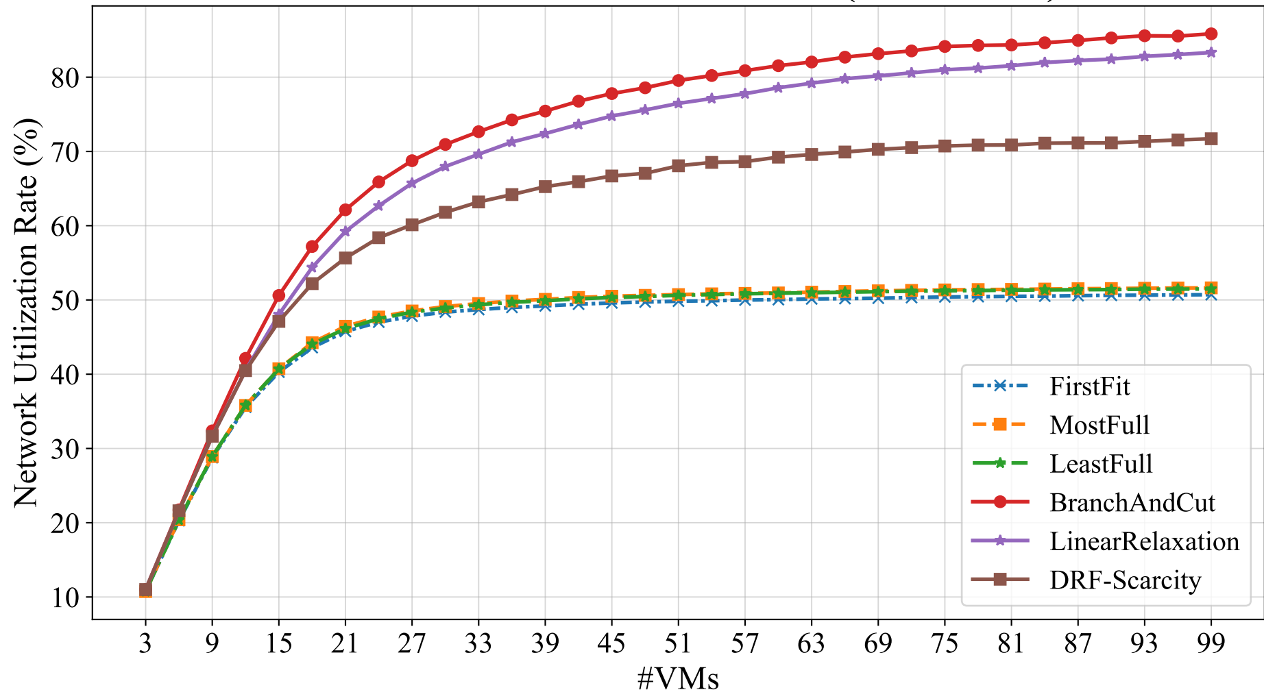
Network Utilization Rate vs #VMs (over 3 Hosts)
