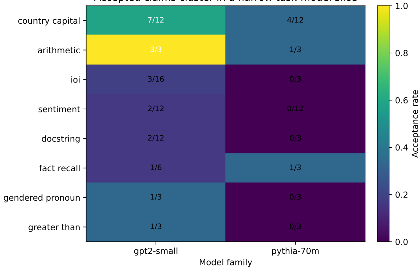
Accepted claims cluster in a narrow task-model slice
