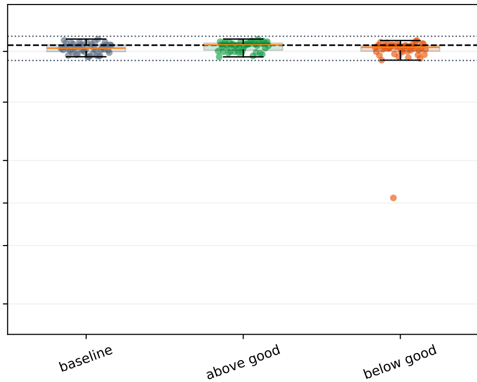
Bounded
