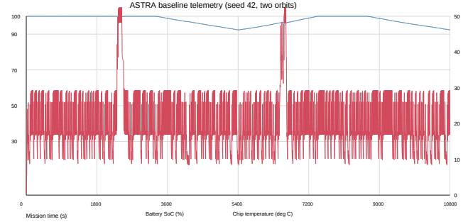
Fig. 1. Heuristic trajectory over two orbits (seed 42). Temperature exceeds the 50°C throttle threshold.
