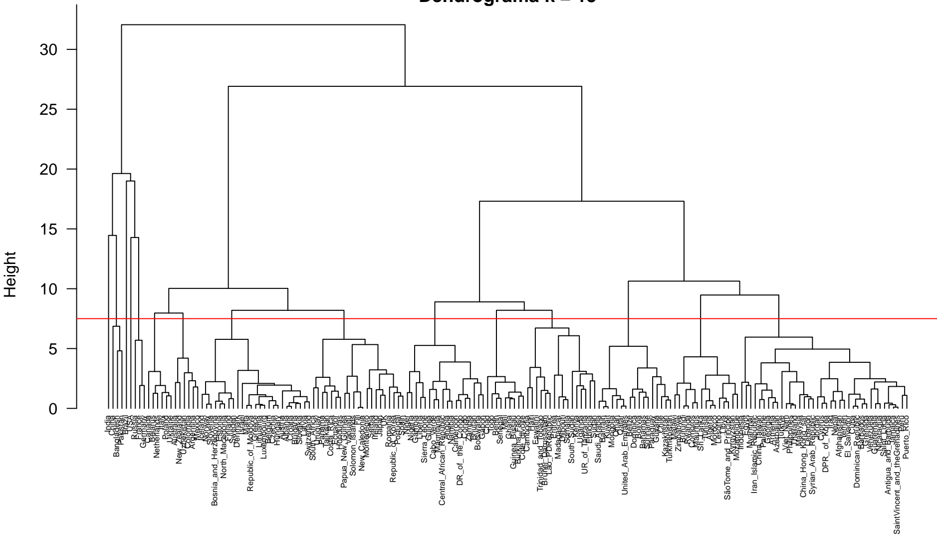
Dendrograma k = 15
