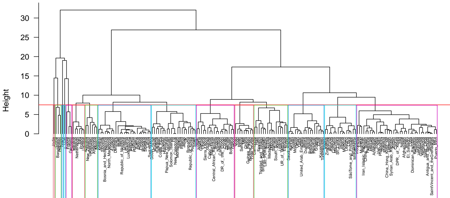
Dendrograma k = 15
