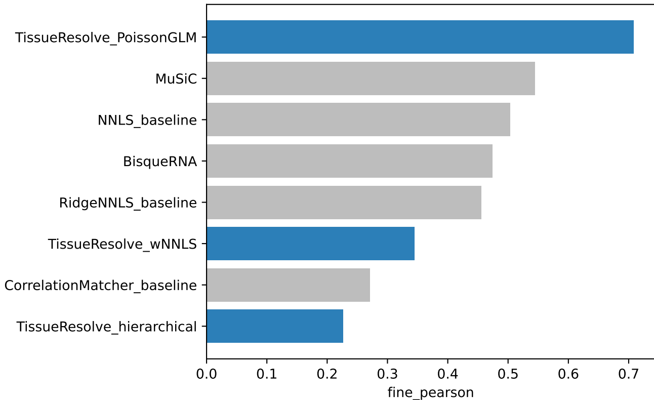
Bulk fine-subpopulation accuracy (Pearson, higher=better)
