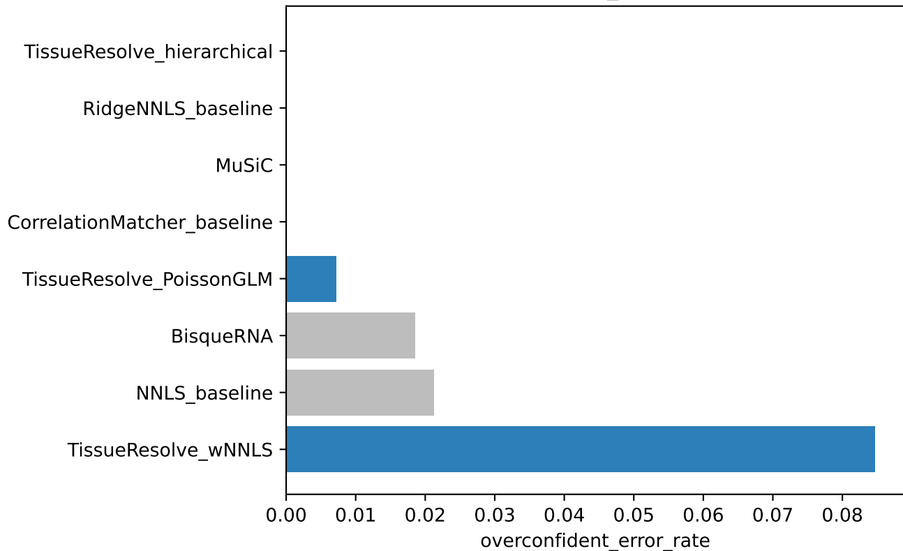
Overconfident fine-state error in GROUP_ONLY/UNRESOLVABLE (lowe
