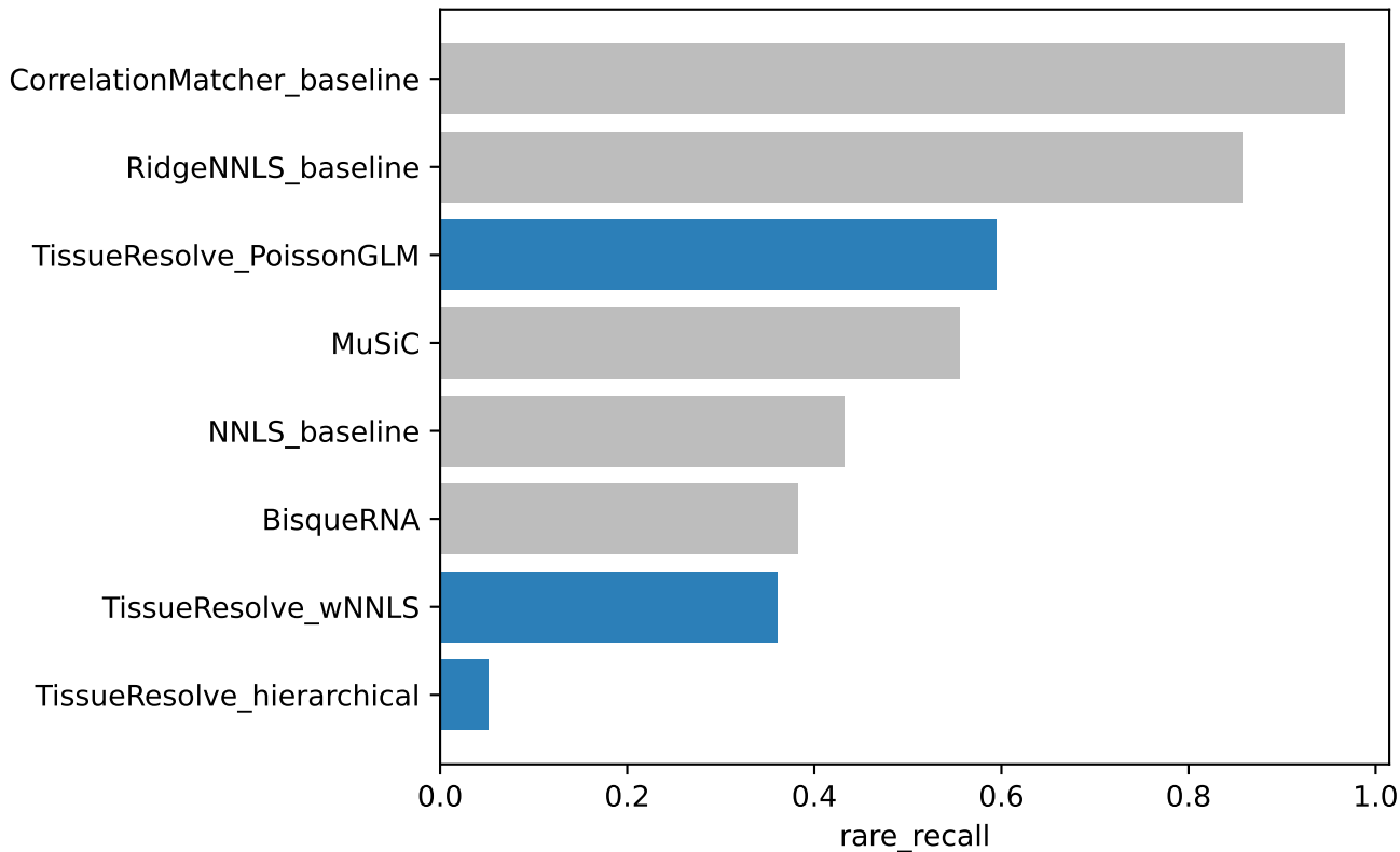
Bulk rare-population recall (higher=better)
