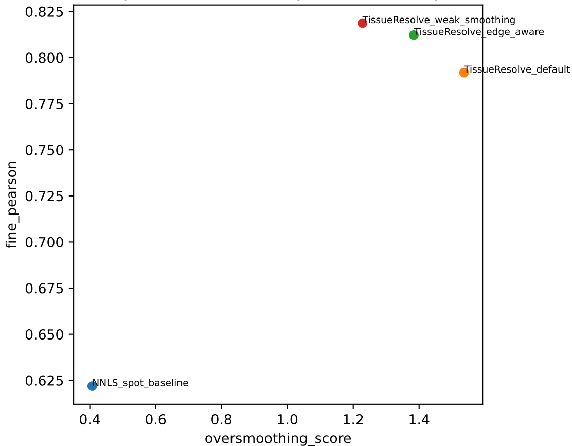
Spatial: oversmoothing vs fine accuracy
