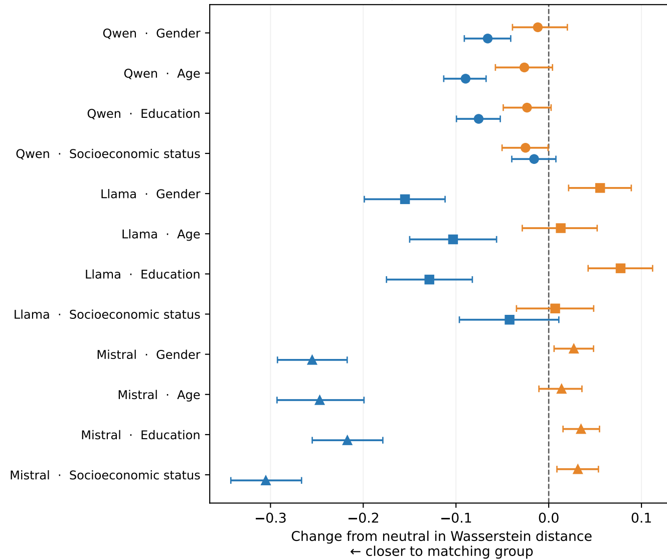
A. Average matching-group distance
