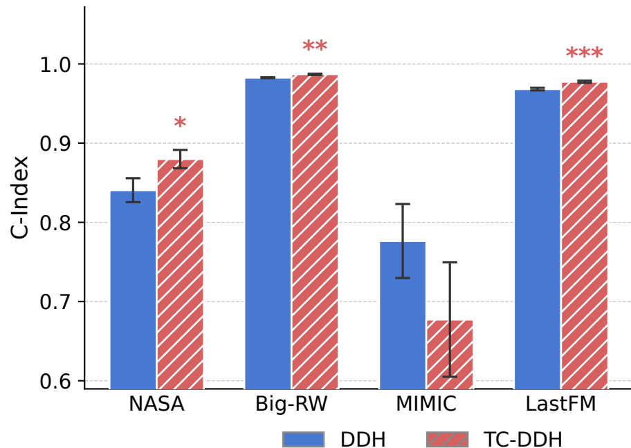
C-Index (↑ higher is better)
