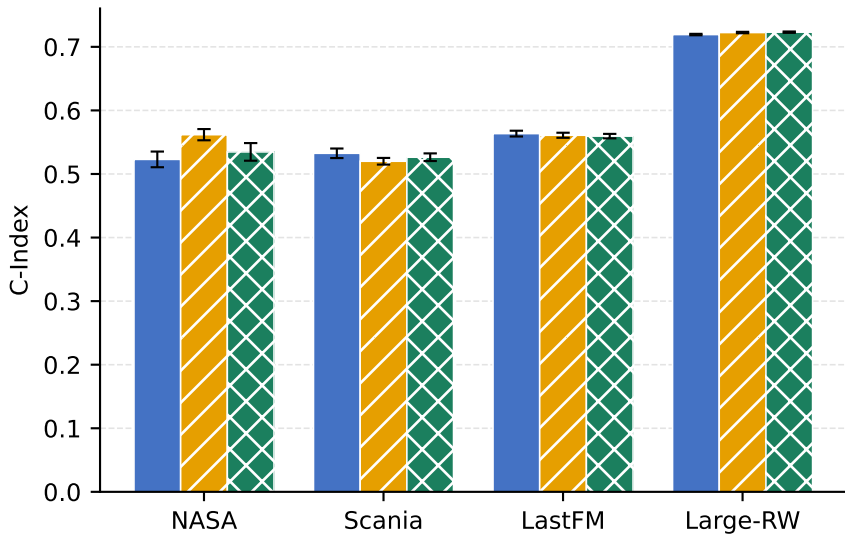
C-Index (higher is better)
