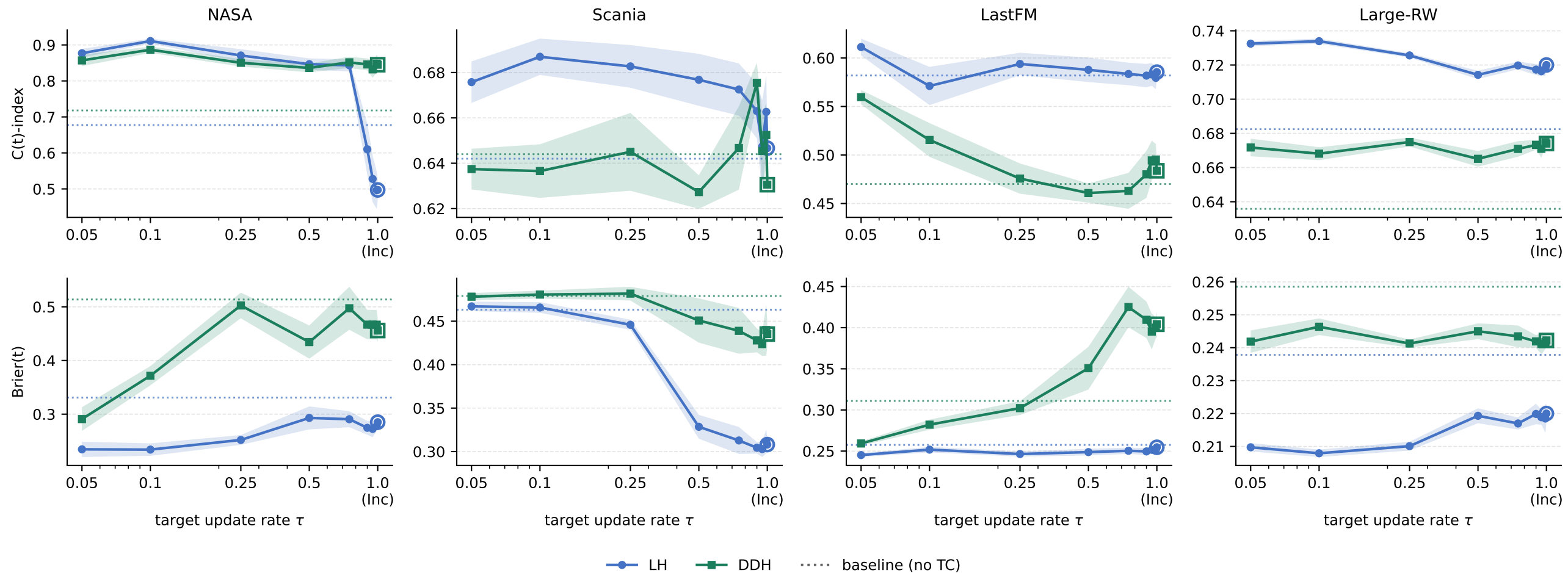
Metric vs target update rate — DDH protocol at the median landmark, \lambda re-tuned per \tau , band = \pm 1 s.e.
