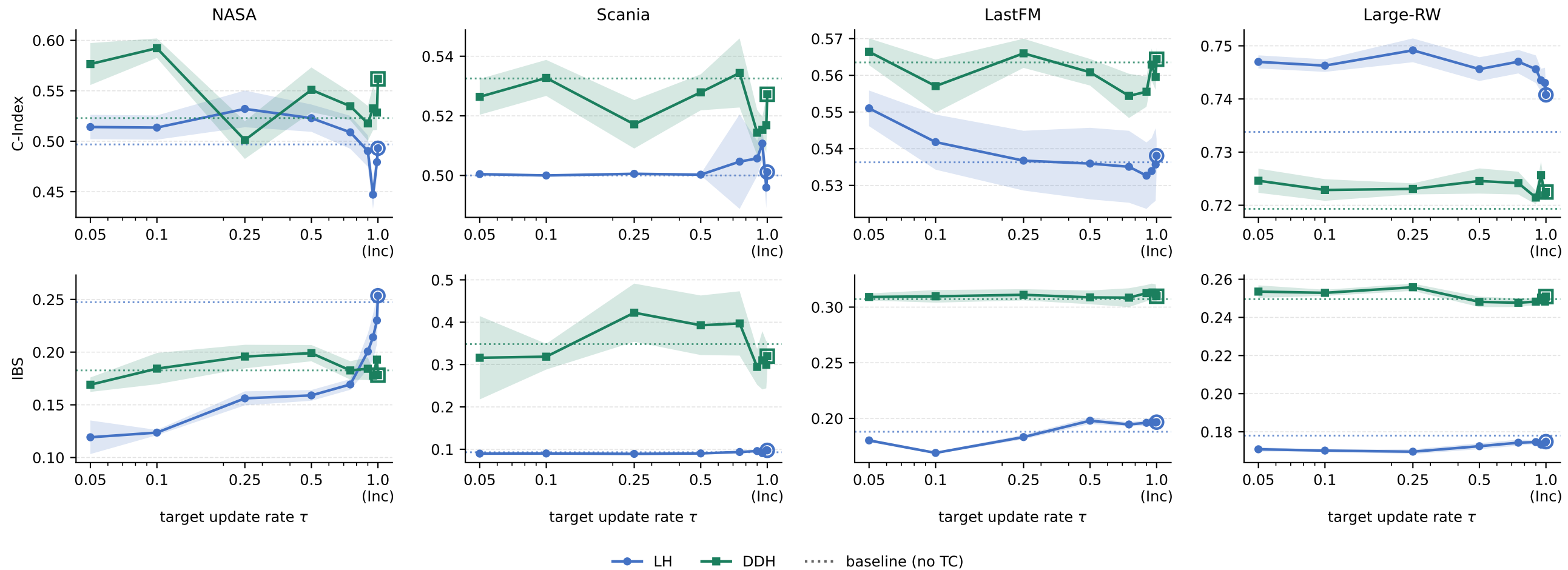
Metric vs target update rate — TCSR protocol (state 0), \lambda re-tuned per \tau , band = \pm 1 s.e.
