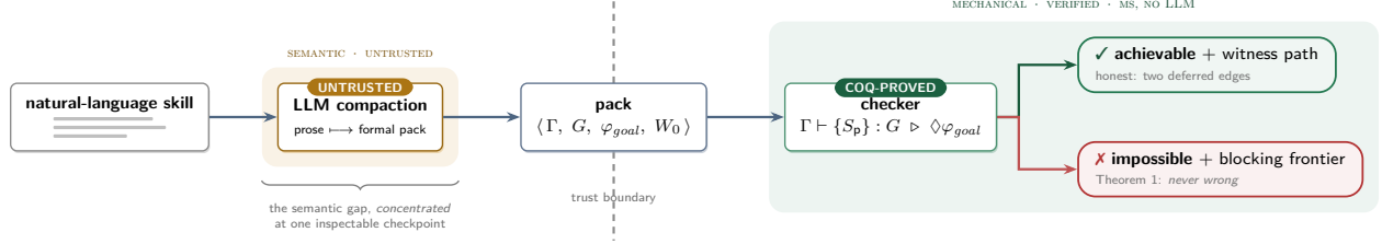
Figure 1: The trust boundary. An untrusted LLM compacts prose into a formal pack; a mechanically verified checker decides achievability over the pack. The verdicts are asymmetric: impossible is sound (Theorem 1), achievable is honest about its two deferred residues (§6.4).
