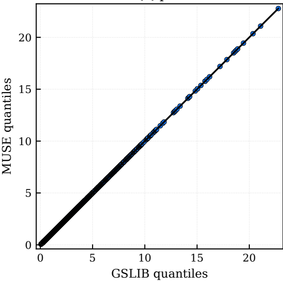
QQ plot
