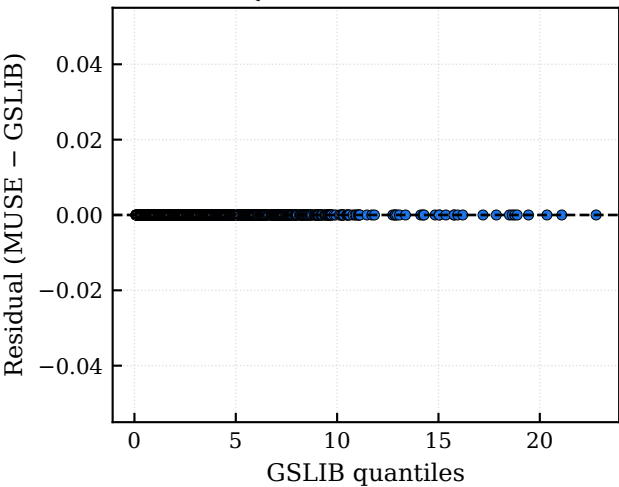
Quantile residuals
