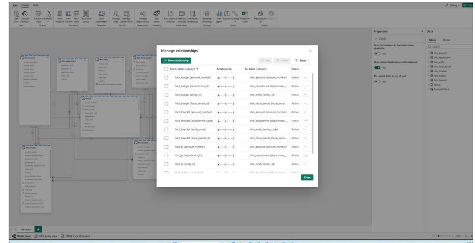
Semantic model - active many-to-one finance relationships.
