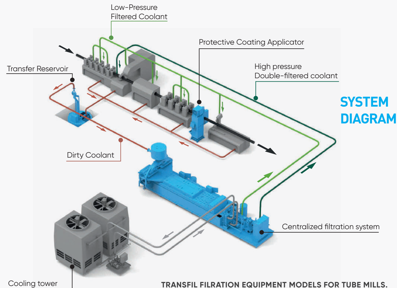
TRANSFIL FILTRATION EQUIPMENT MODELS FOR TUBE MILLS.
