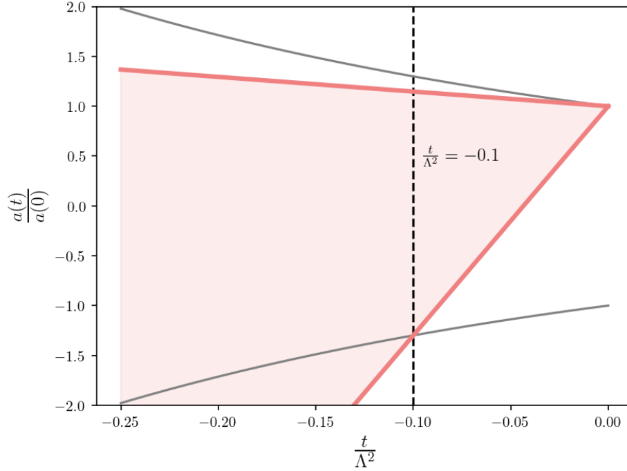
Figure 4.34: Bounds on a(t) for m^2/\Lambda^2 = 0.1 , -t/\Lambda^2 = 0.1 and two subtractions. The red region indicates the range of values of a(t)/a_0 consistent with Equation (4.33). The upper boundary corresponds to the minimum allowed value of m , while the lower boundary corresponds to the maximum allowed value.
