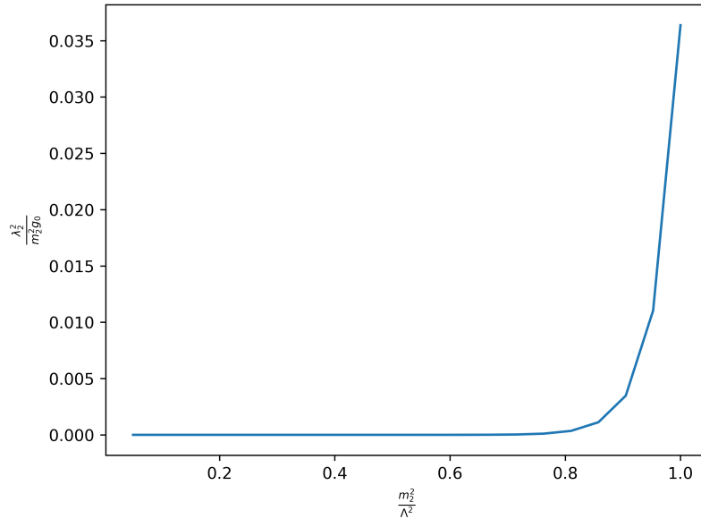
Figure 3.35: Bounds for a massive spin 2 resonance and massless external legs.
