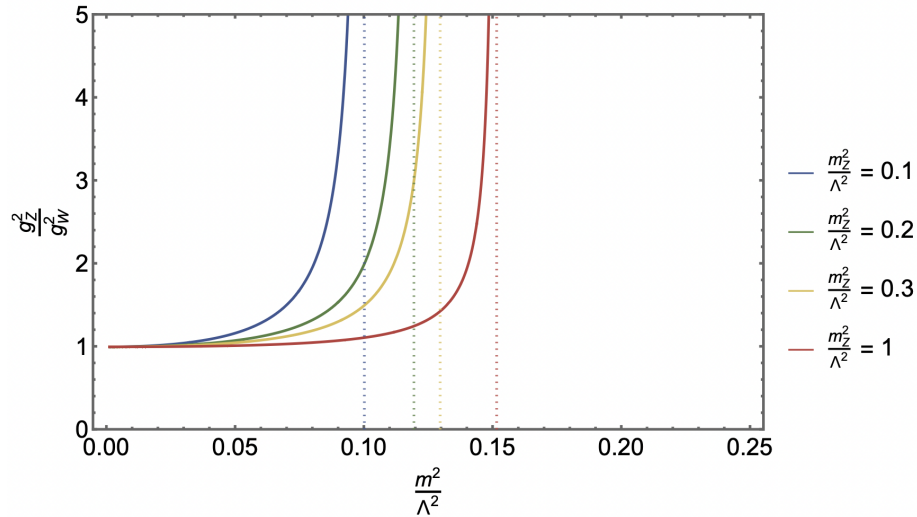
Figure 5.20: Upper bound in g_Z for different values of m^2 and m_Z^2 , only including dimension 4 operators and assuming the isospin-2 amplitude is analytical. The dashed lines represent the value of m^2 starting from which the theory is not consistent, as it gives g_Z < 0 .
