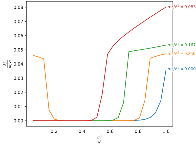
Figure 3.38: Bounds for a massive spin 2 resonance and a massive spin 0 resonance with massive scalar external legs, shown for different values of the external mass. The spin 0 resonance and the external legs have equal mass. The blue line represents the bound in the absence of spin 0 exchange.
