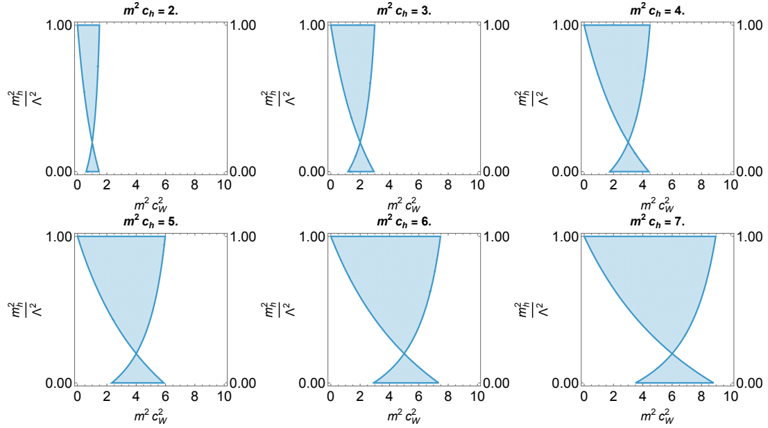
Figure 5.17: Regions of parameter space compatible with the positivity bounds for t = 0.1 \Lambda^2 , including dimension 4 and dimension 6 operators and assuming that c_{HW} + c_W = 1/(2m^2) and c_W \geq 0 .
