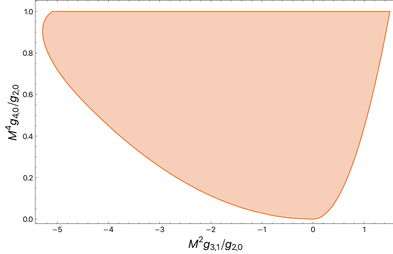
Figure 2.49: Allowed region for the \tilde{g}_3 and \tilde{g}_4 Wilson coefficient in a theory for a massless scalar.
