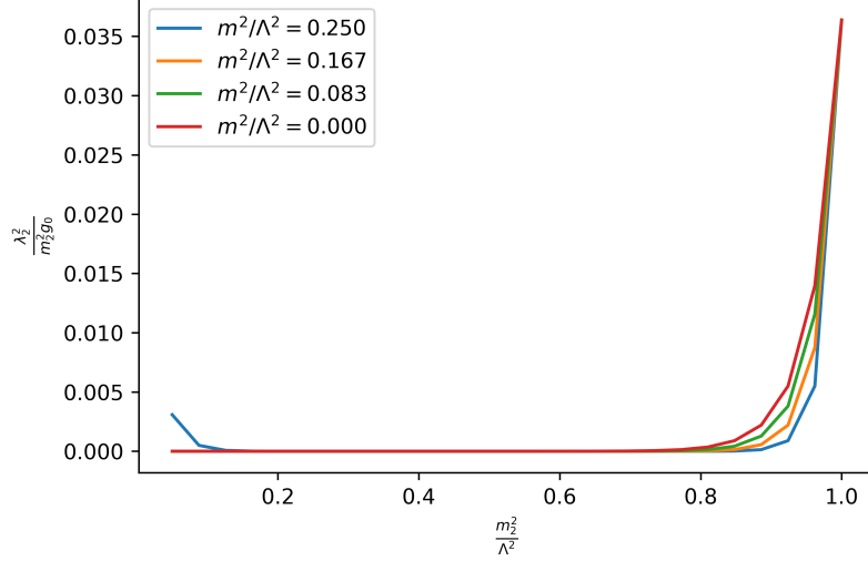
Figure 3.36: Bounds for a massive spin 2 resonance and massive scalar external legs.
