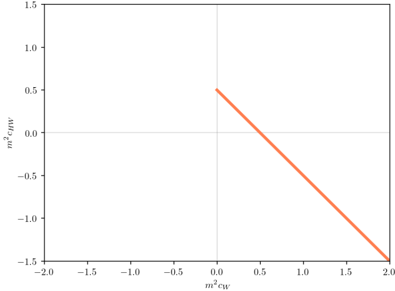
Figure 5.14: Region in the (c_W, c_{HW}) parameter space for which there are no bounds in the spectrum.
