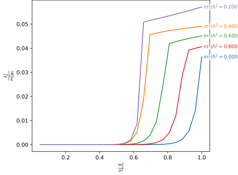
Figure 3.37: Bounds for a massive spin 2 resonance and a massive spin 0 resonance with massless scalar external legs, shown for different values of the spin 0 mass. The blue line represents the bound in the absence of spin 0 exchange.
