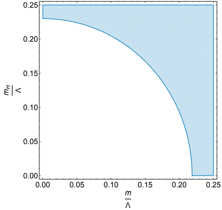
Figure 5.22: Allowed region for m and m_H independently of the value of the 6 dimensional coefficients, assuming the isospin-2 amplitude is analytical.
