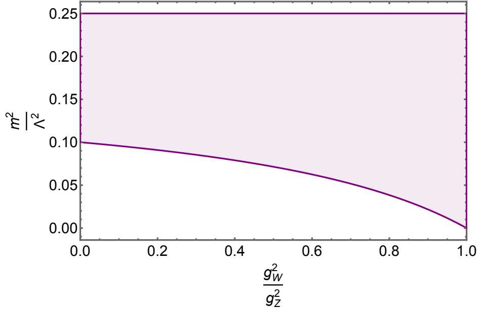
Figure 5.21: Allowed region for m^2 for different values in g_Z , only including dimension 4 operators and assuming the isospin-2 amplitude is analytical.
