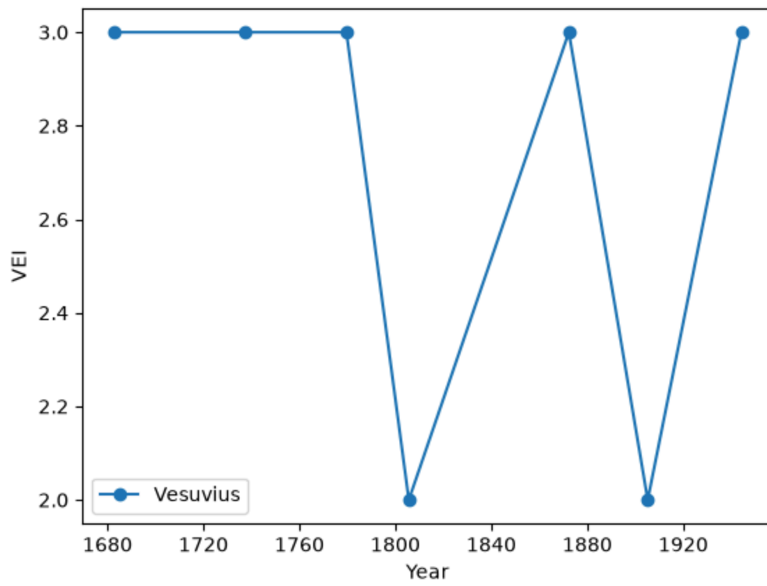
Vesuvius
