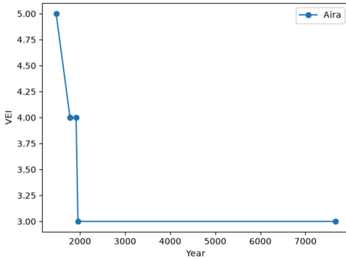
Aira
