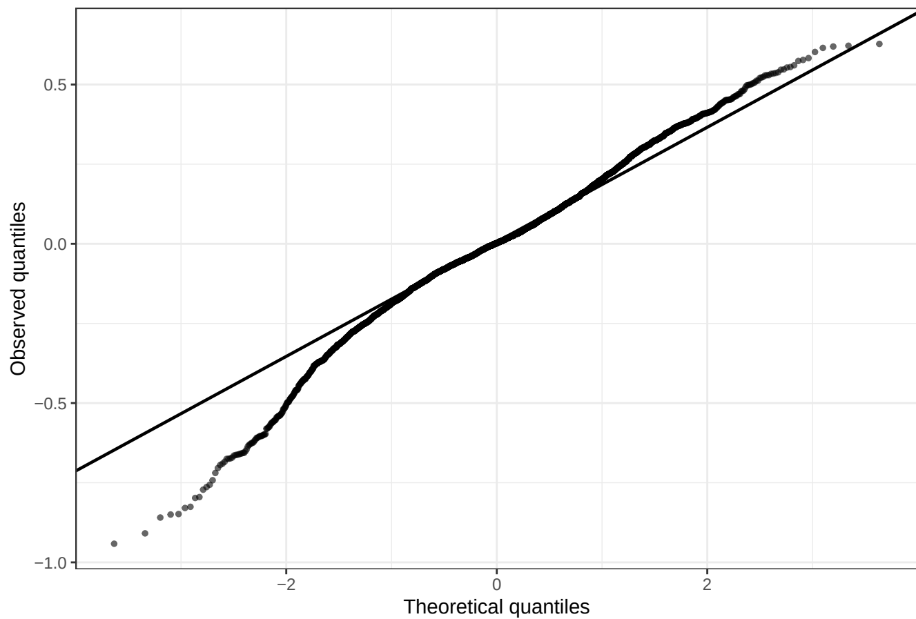
Normal Q-Q plot of recruitment residuals
