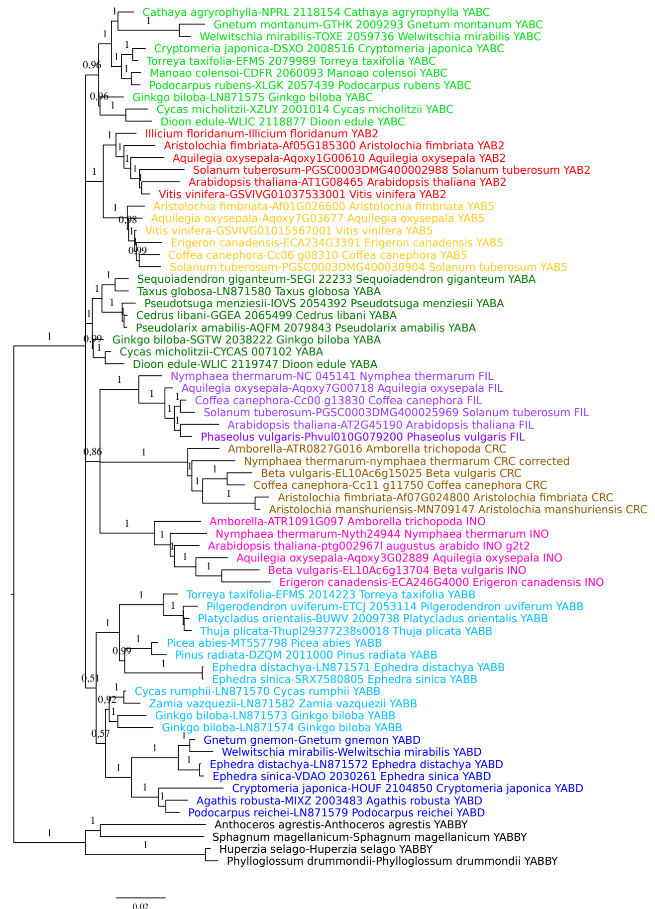
b) Majority consensus inferred from 100 reconciled scenarios based on BALi-Phy reconstructions on complete sequences with codon encoding
