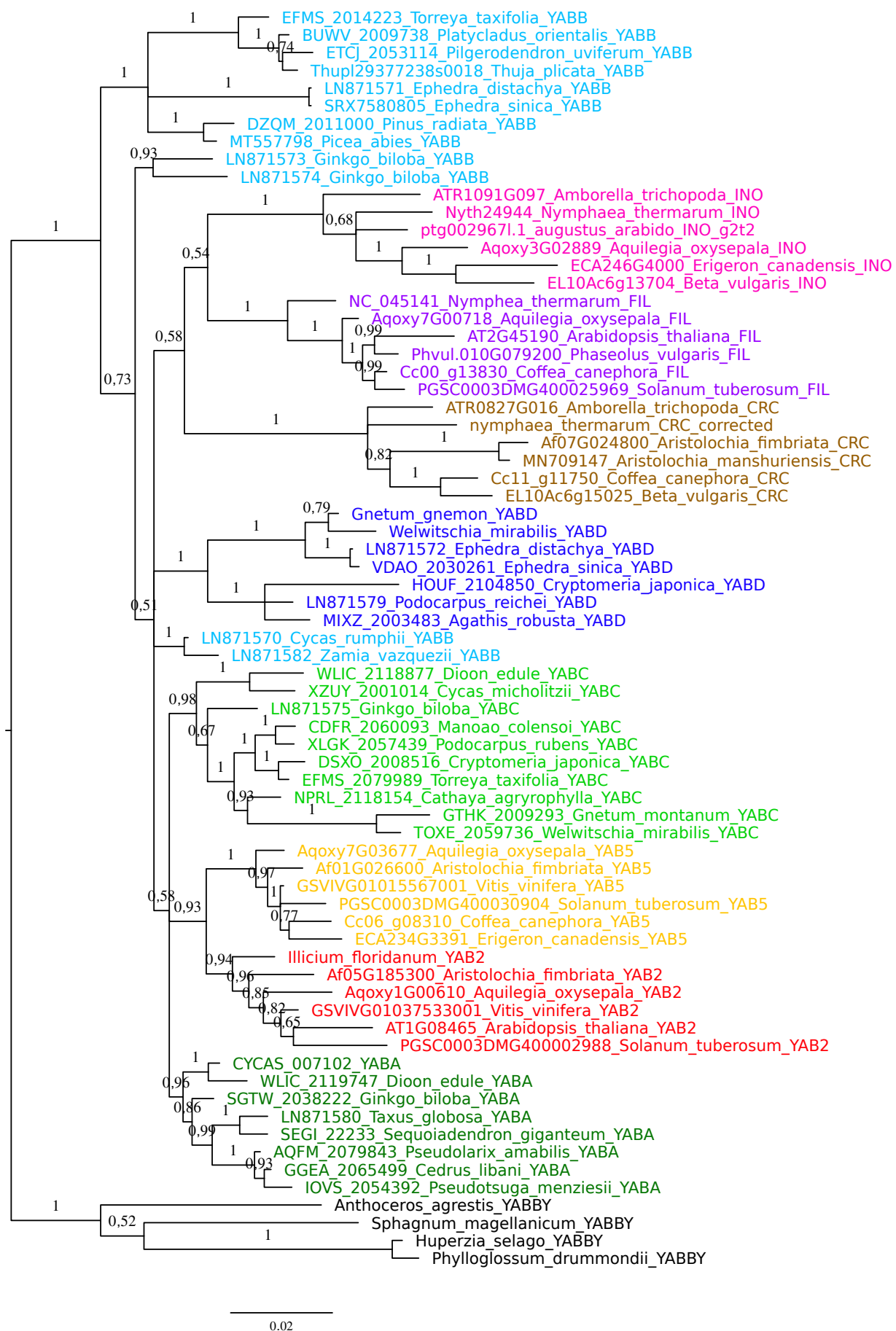
a) Majority consensus tree inferred from BALi-Phy reconstructions on complete sequences with aa encoding
