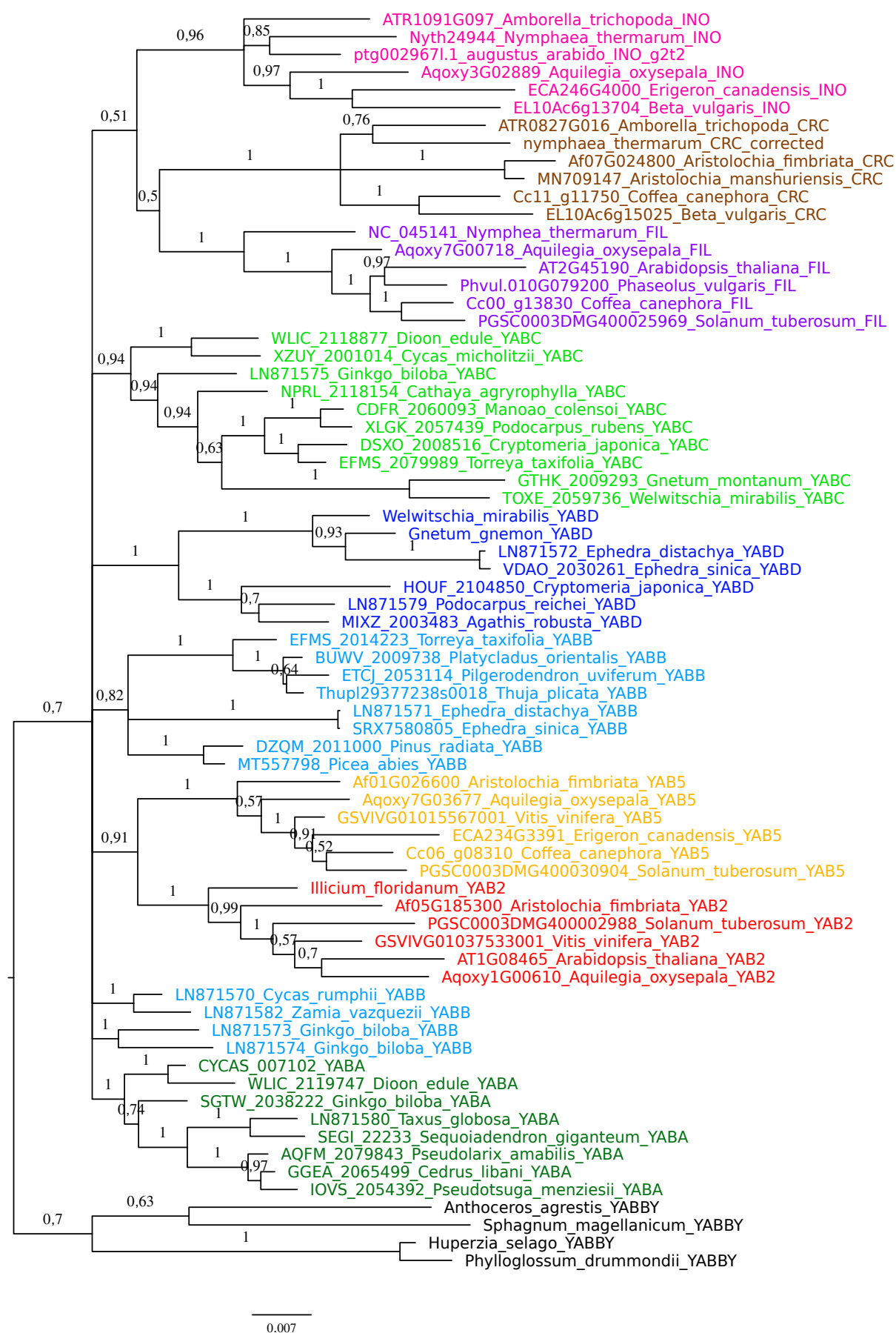
a) Majority consensus inferred from BALi-Phy reconstructions on complete sequences with codon encoding
