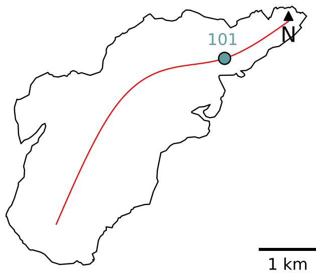
Allalin
