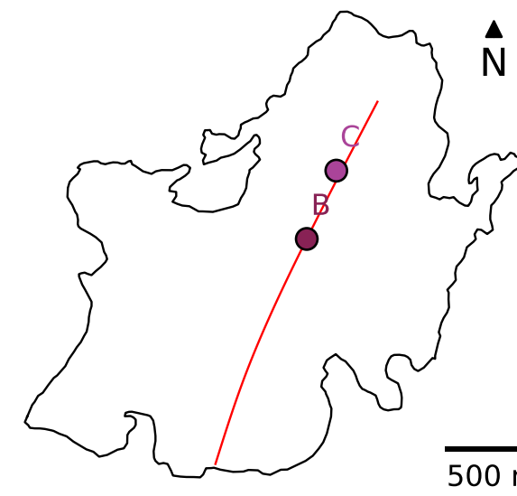
Saint-Sorlin
