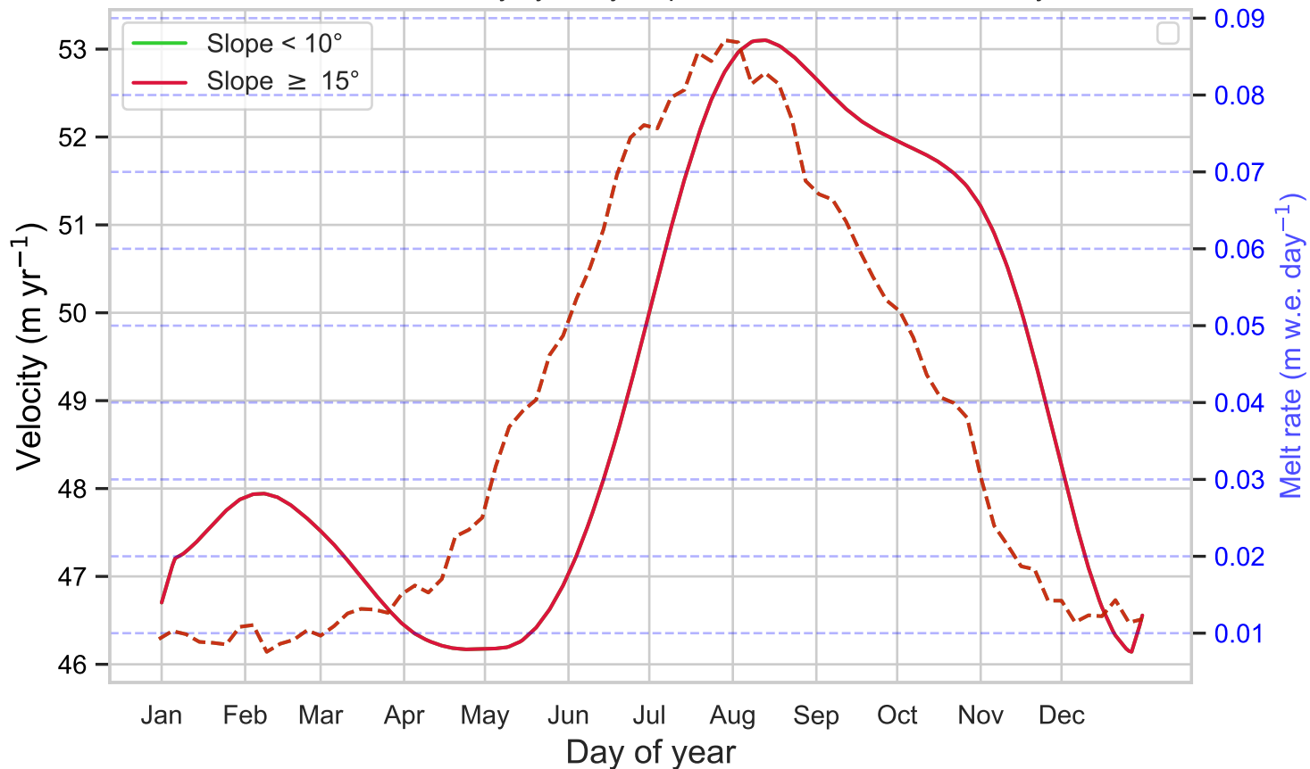
Mean seasonal velocity cycle by slope class & annual melt rate cycle
