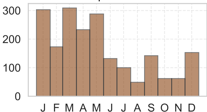
Slope 24–30°
