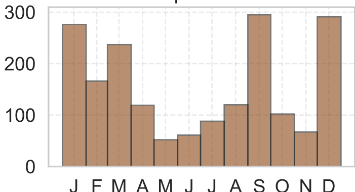
Slope 12–18°
