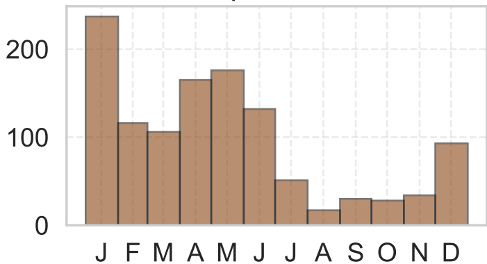
Slope 30–36°
