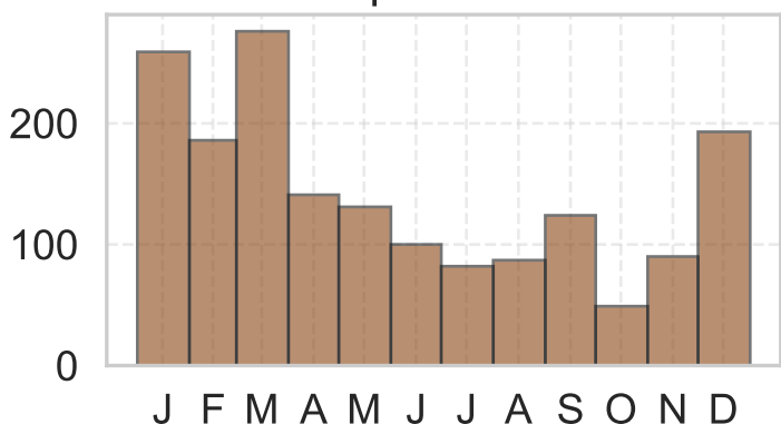
Slope 18–24°
