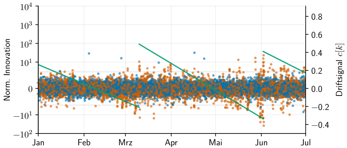
(b) Kalman-Filter
