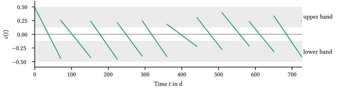
Figure 2. Drift signal c(t) of IDV(29).
