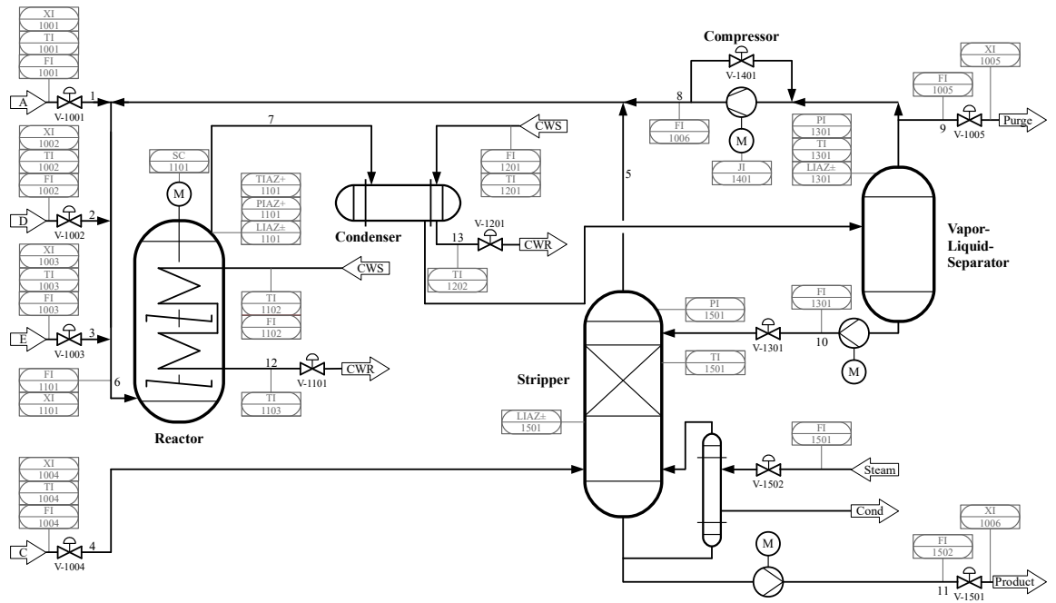
Figure 1. Flowsheet of the TEP with its five main units, redrawn in monochrome after [11].
