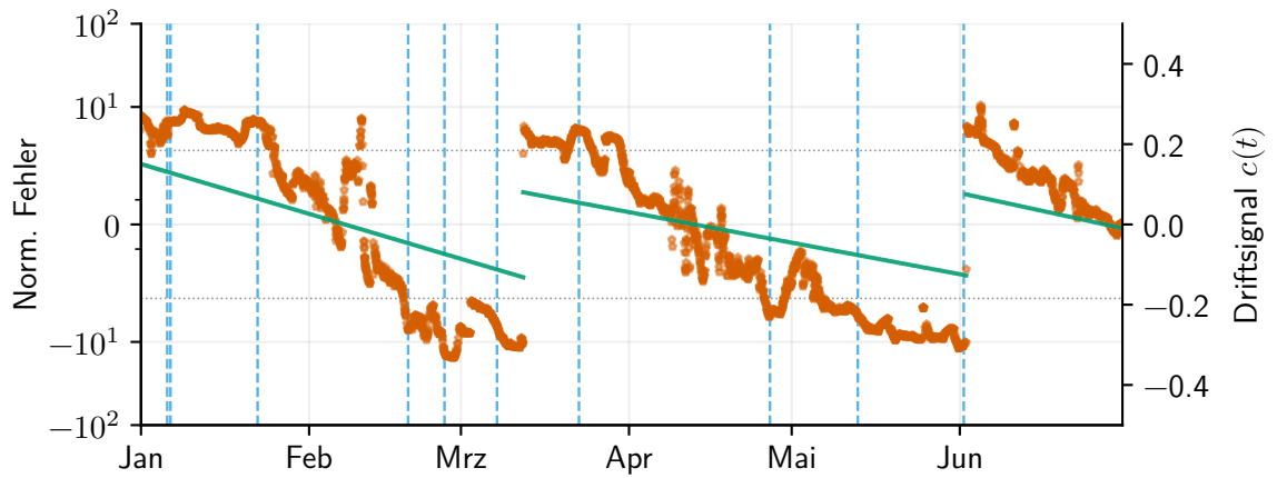
(b) DDM
