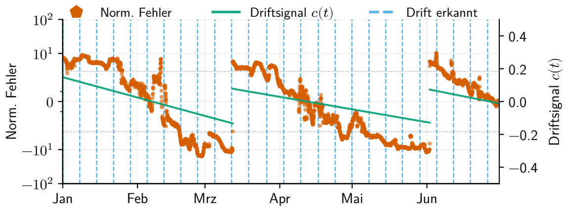
(a) KSWIN
