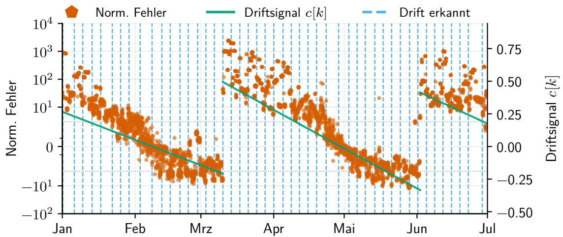
(a) KSWIN
