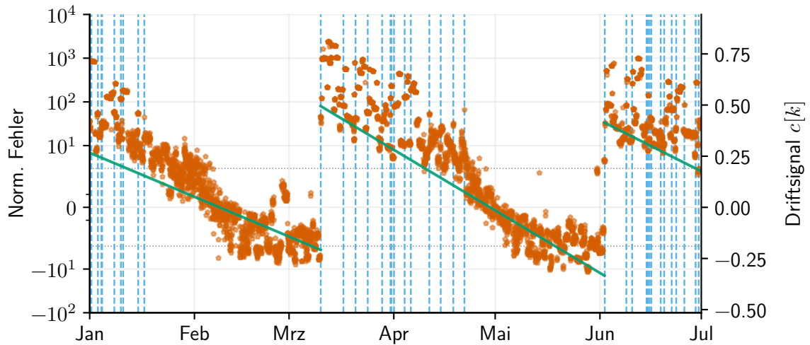
(b) DDM
