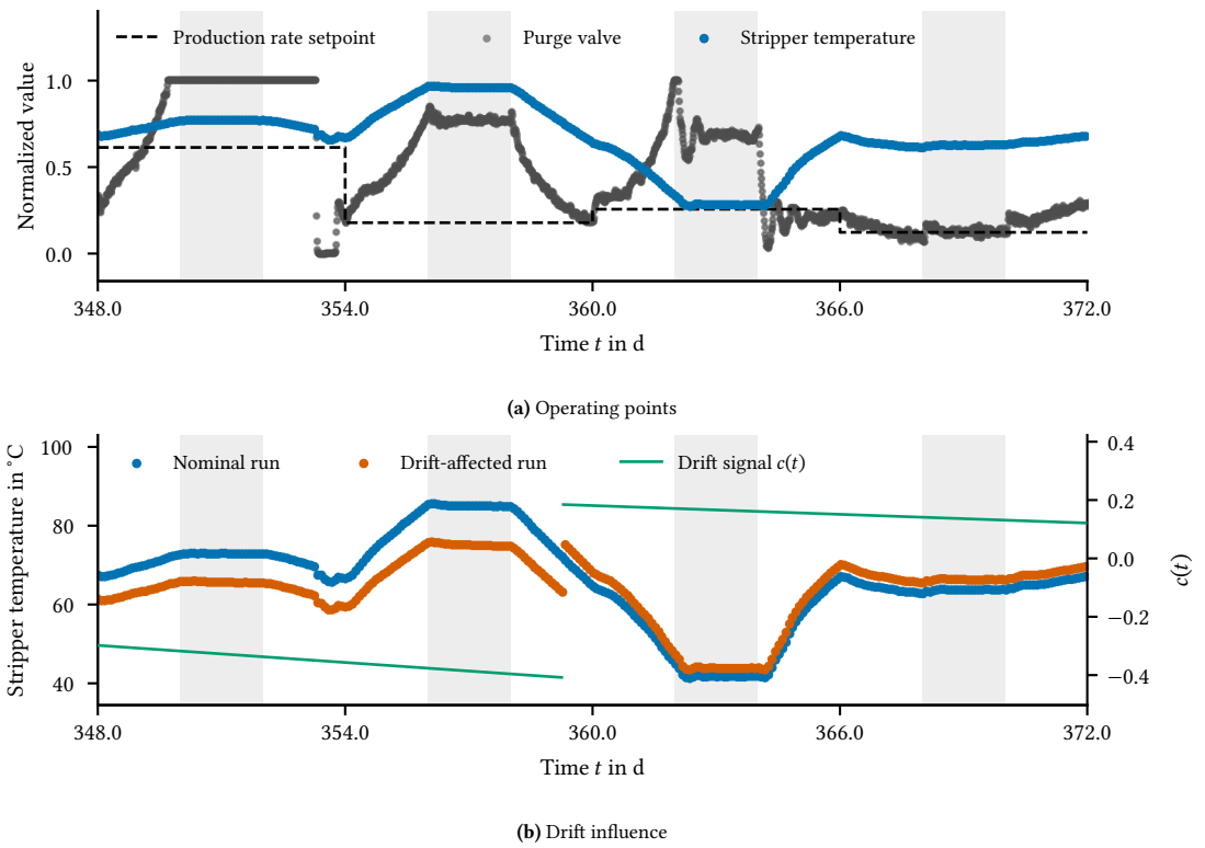
Figure 3. Excerpt of the generated data stream over four operating points.
