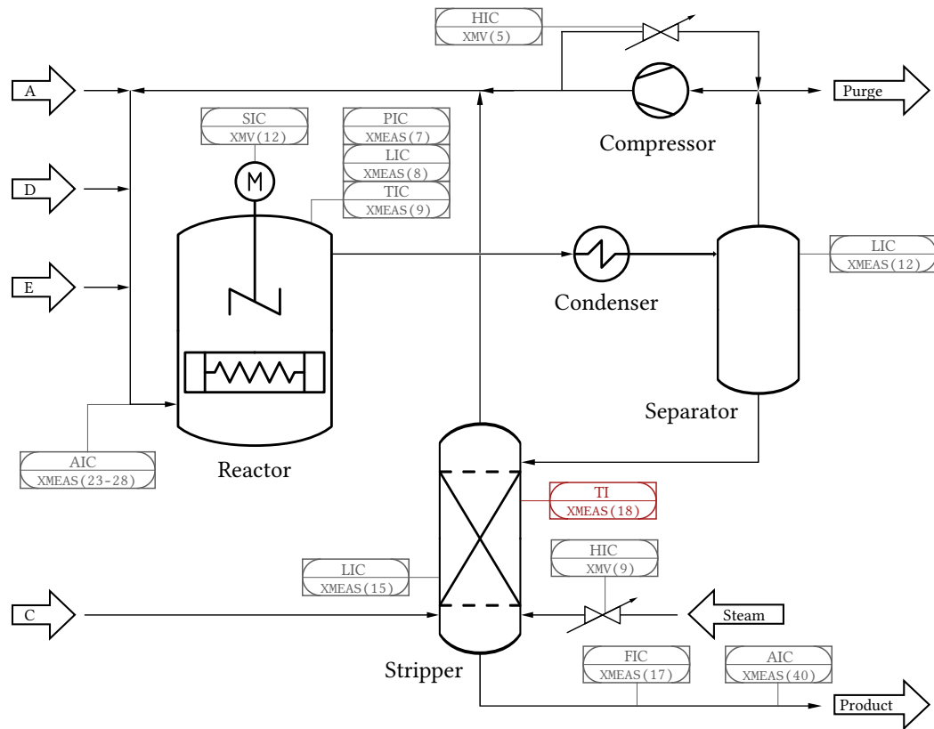
Figure 1. Flowsheet of the TEP with its five main units, after [8].
