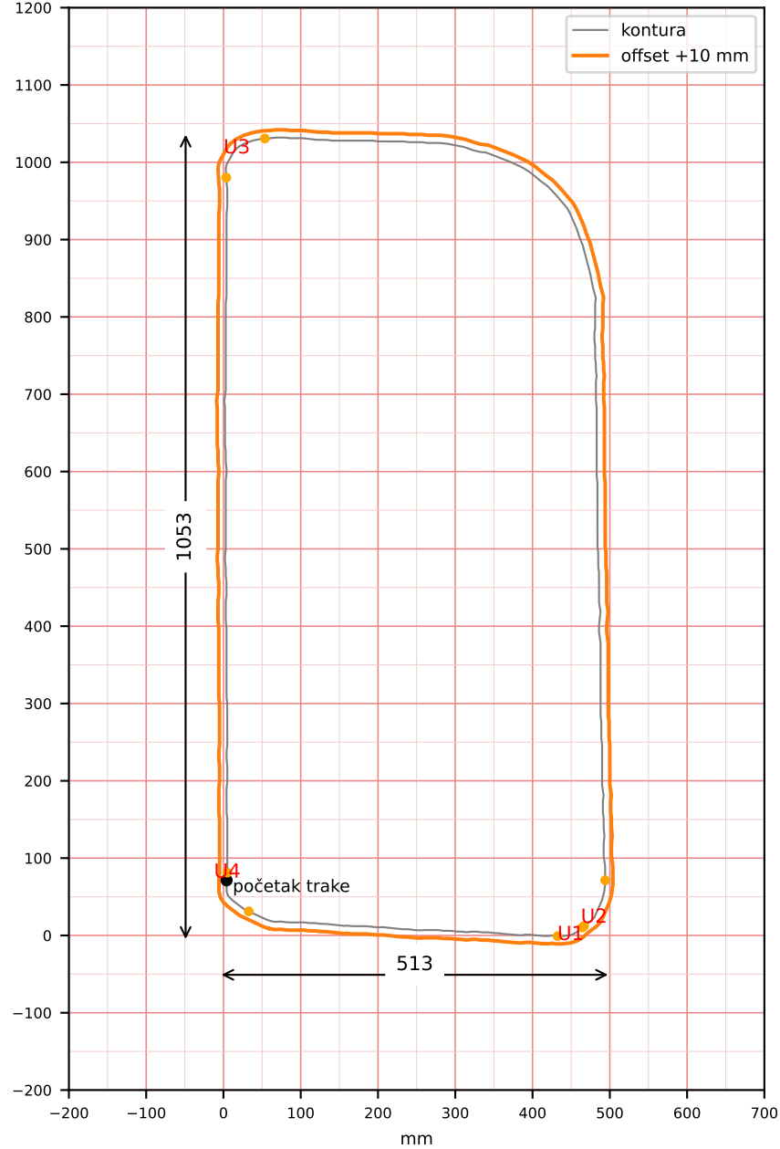
MALA KUPA STOLA - offset +10 mm (gabarit 513 x 1053 mm); traka 90 x 2850 mm
