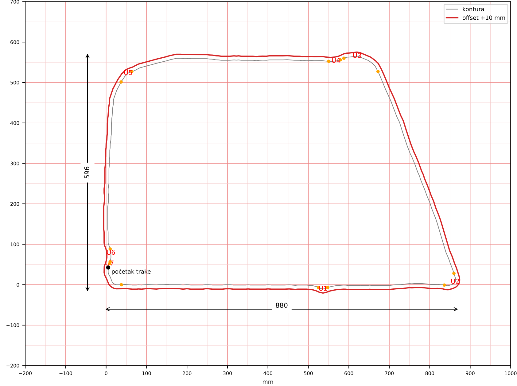
1F LICE - offset +10 mm (gabarit 880 x 596 mm); traka 90 x 2588 mm
