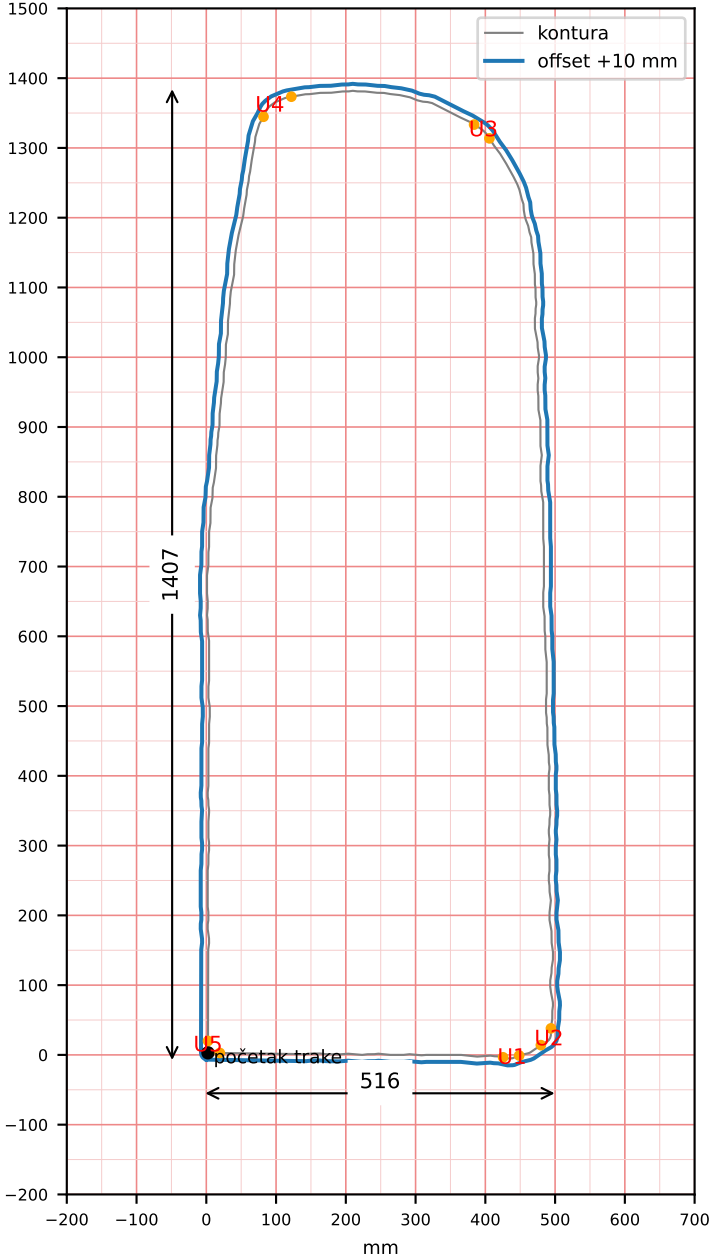
KLUP LICE - offset +10 mm (gabarit 516 x 1407 mm); traka 90 x 3514 mm
