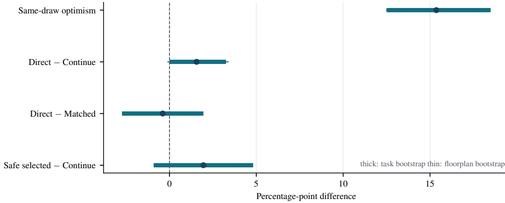
Figure 3: Confirmation effects on ALFWorld. Dots show planned-task means; thick and thin intervals show task- and floorplan-bootstrap 95% intervals. Reported adjusted p values use the prespecified group sign-flip tests and Holm correction.
