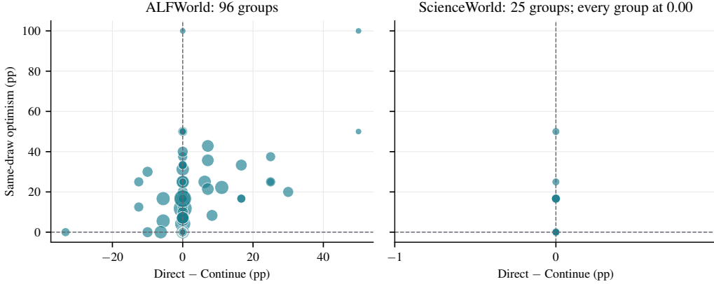
Figure 4: Group-level measurement and policy effects. Each point is a complete floorplan or task-family group; area is proportional to its task count. Vertical position is same-draw optimism and horizontal position is Direct minus Continue; a group in the upper left shows optimism from the outcome-informed selector while the deployable controller loses utility. Every ScienceWorld group lies on the vertical zero-effect line. Dashed lines mark zero.
