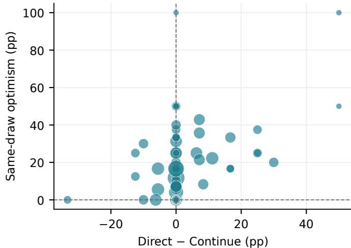
ALFWorld: 96 groups
