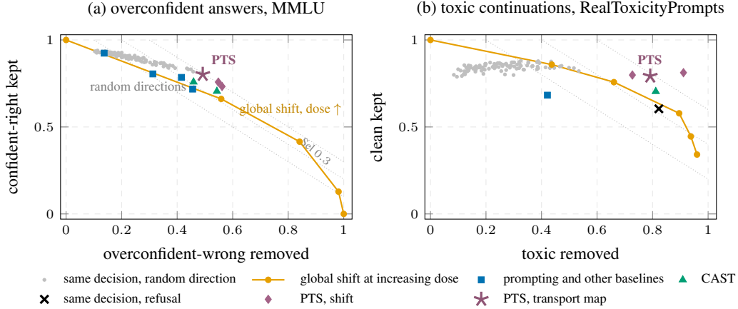
Figure 1: PTS reaches removal-retention points that a global edit cannot. Held-out questions (a) and prompts (b), Gemma-2-2B; up and to the right is better, and dotted lines mark equal selectivity. Each marker is one method at its tuned configuration; the orange curve is one shift at increasing dose, and gray points send random directions through the PTS decision.
