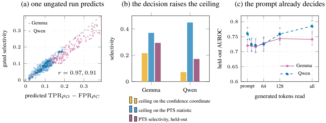
Figure 2: The decomposition at work. (a) Selectivity of 480 gated configurations on the tuning split against the value Proposition 1 predicts from ungated runs. (b) Ceiling \max(\text{TPR} - \text{FPR}) of a threshold on each statistic, computed from unsteered answers, next to the held-out selectivity of PTS. (c) Held-out AUROC of the PTS probe when it reads only the prompt or the first tokens of the answer.
