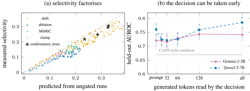
Figure 2: The decision is the lever, and it can be taken early. (a) Each point is a decision–action–threshold combination on the Gemma tuning split (240 in total). The horizontal axis is \text{TPR}_{\rho_O} - \text{FPR}_{\rho_C} computed from the ungated run of the action; the vertical axis is the selectivity of the gated edit. Stars are the four gated arms of the confirmatory split, measured on real runs. (b) AUROC between OCW and CR on the 3,000 confirmatory questions of a probe that reads the prompt, the first t generated tokens, or the whole answer; bars are 95% bootstrap intervals, and the dotted line is the trace direction used by the CAST-style condition.
