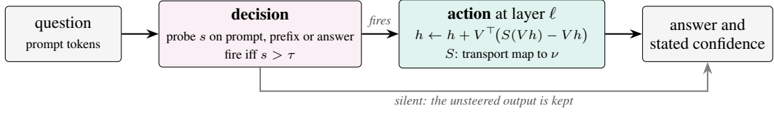
Figure 1: PTS separates when to edit from how to edit. A probe reads the input and decides whether to act; the action moves the projection Vh of the residual stream to a target law and leaves the orthogonal complement unchanged. The selectivity of the combination is the decision’s error rates weighted by the action’s conversion rates of the two states (Prop. 1).
